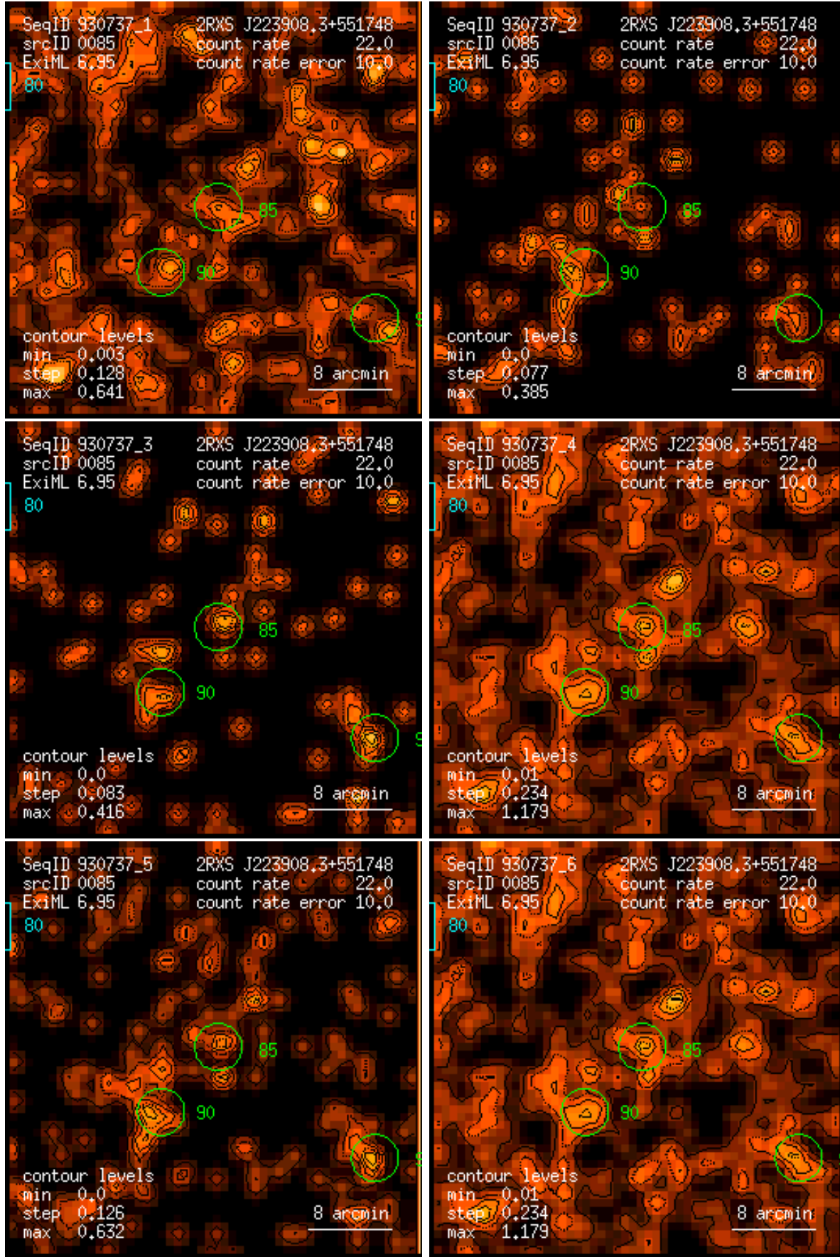
Figure 85: RASS 930737: detection 0085: band rate images, Gaussian filter: (1) PSPC channels 11 – 41, (2) 52 – 90, (3) 91 – 201, (4) 11 – 235, (5) 52 – 201, (6) 11 – 201. Broad band rates in counts/ks. Band rate contour levels in counts/ks/arcmin 2 .
