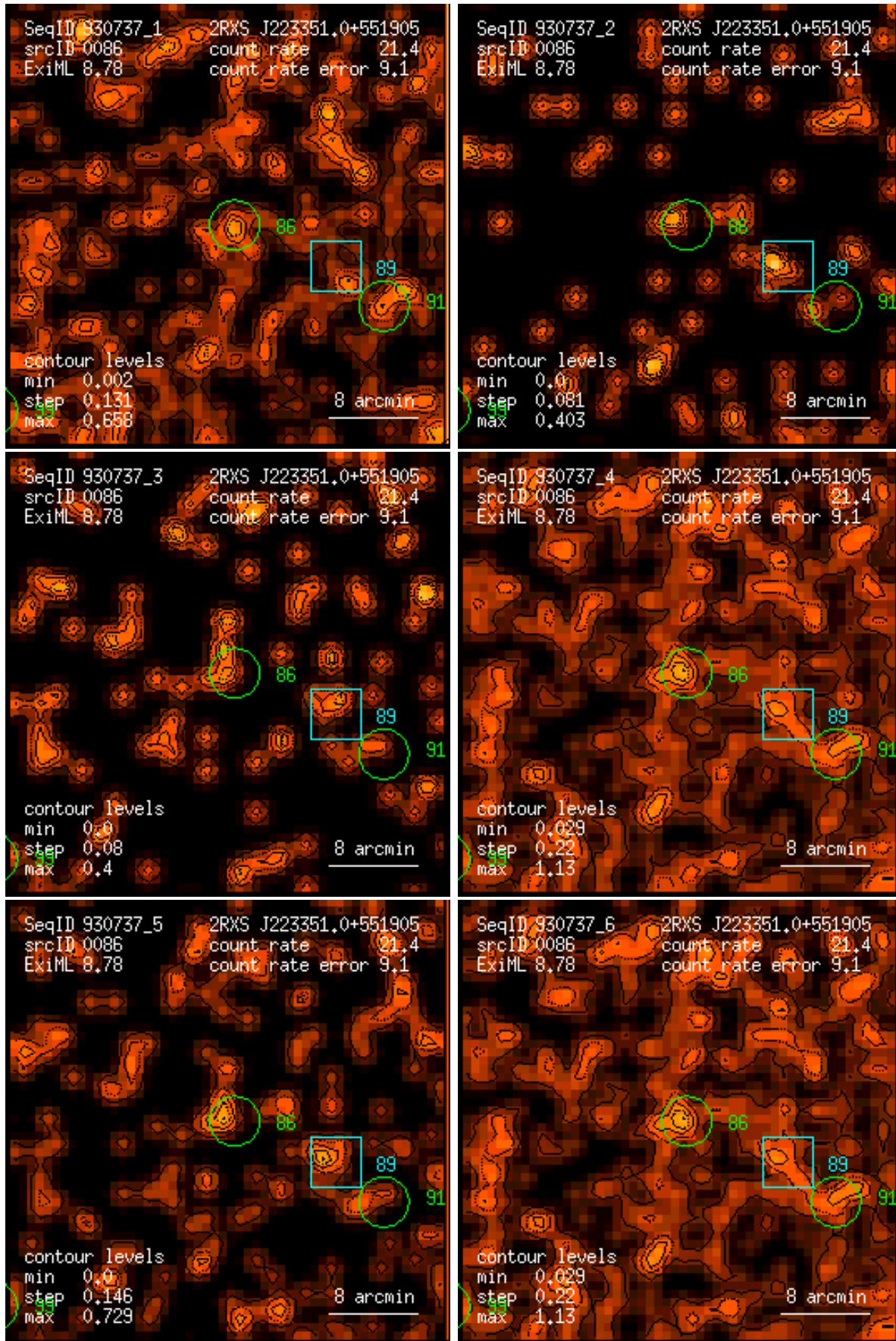
Figure 86: RASS 930737: detection 0086: band rate images, Gaussian filter: (1) PSPC channels 11 – 41, (2) 52 – 90, (3) 91 – 201, (4) 11 – 235, (5) 52 – 201, (6) 11 – 201. Broad band rates in counts/ks. Band rate contour levels in counts/ks/arcmin 2 .
