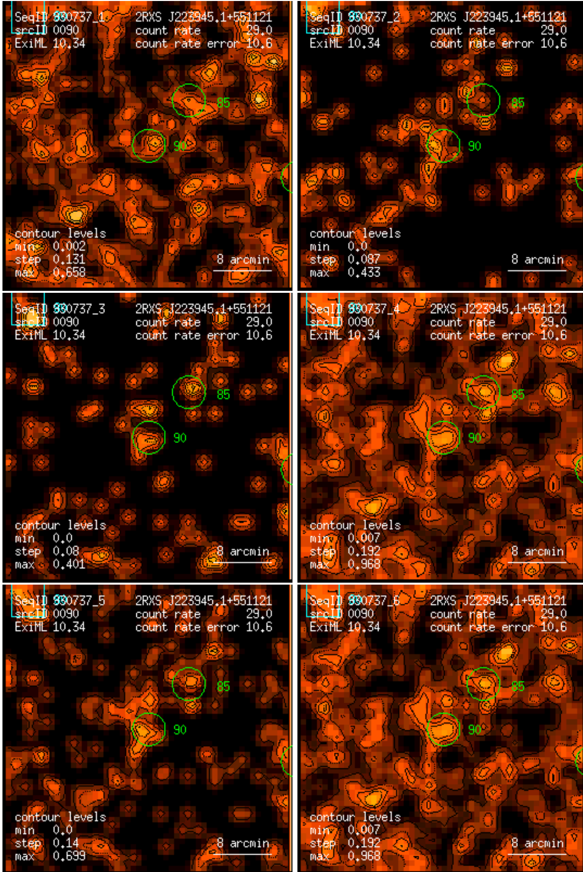
Figure 90: RASS 930737: detection 0090: band rate images, Gaussian filter: (1) PSPC channels 11 – 41, (2) 52 – 90, (3) 91 – 201, (4) 11 – 235, (5) 52 – 201, (6) 11 – 201. Broad band rates in counts/ks. Band rate contour levels in counts/ks/arcmin 2 .
