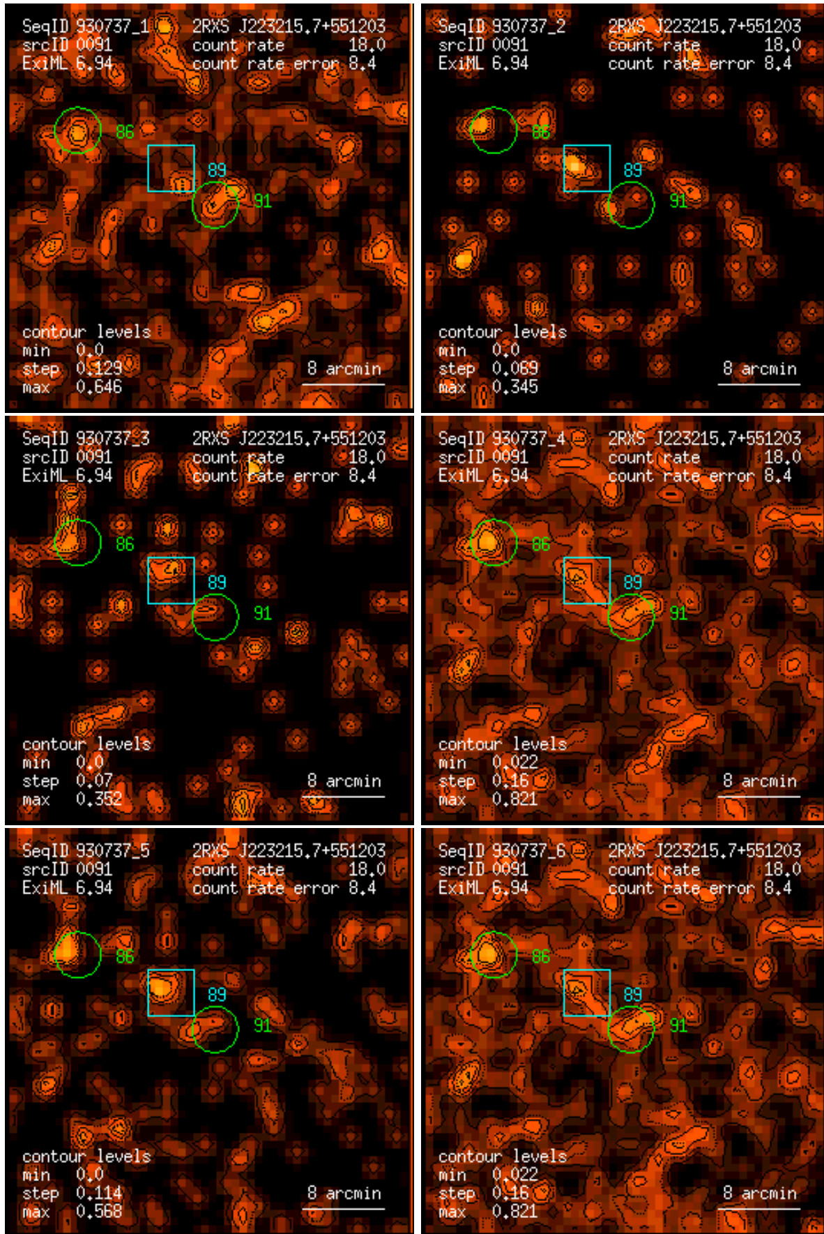
Figure 91: RASS 930737: detection 0091: band rate images, Gaussian filter: (1) PSPC channels 11 – 41, (2) 52 – 90, (3) 91 – 201, (4) 11 – 235, (5) 52 – 201, (6) 11 – 201. Broad band rates in counts/ks. Band rate contour levels in counts/ks/arcmin 2 .
