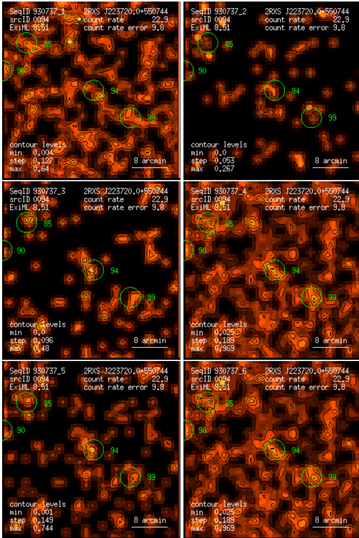
Figure 94: RASS 930737: detection 0094: band rate images, Gaussian filter: (1) PSPC channels 11 – 41, (2) 52 – 90, (3) 91 – 201, (4) 11 – 235, (5) 52 – 201, (6) 11 – 201. Broad band rates in counts/ks. Band rate contour levels in counts/ks/arcmin 2 .
