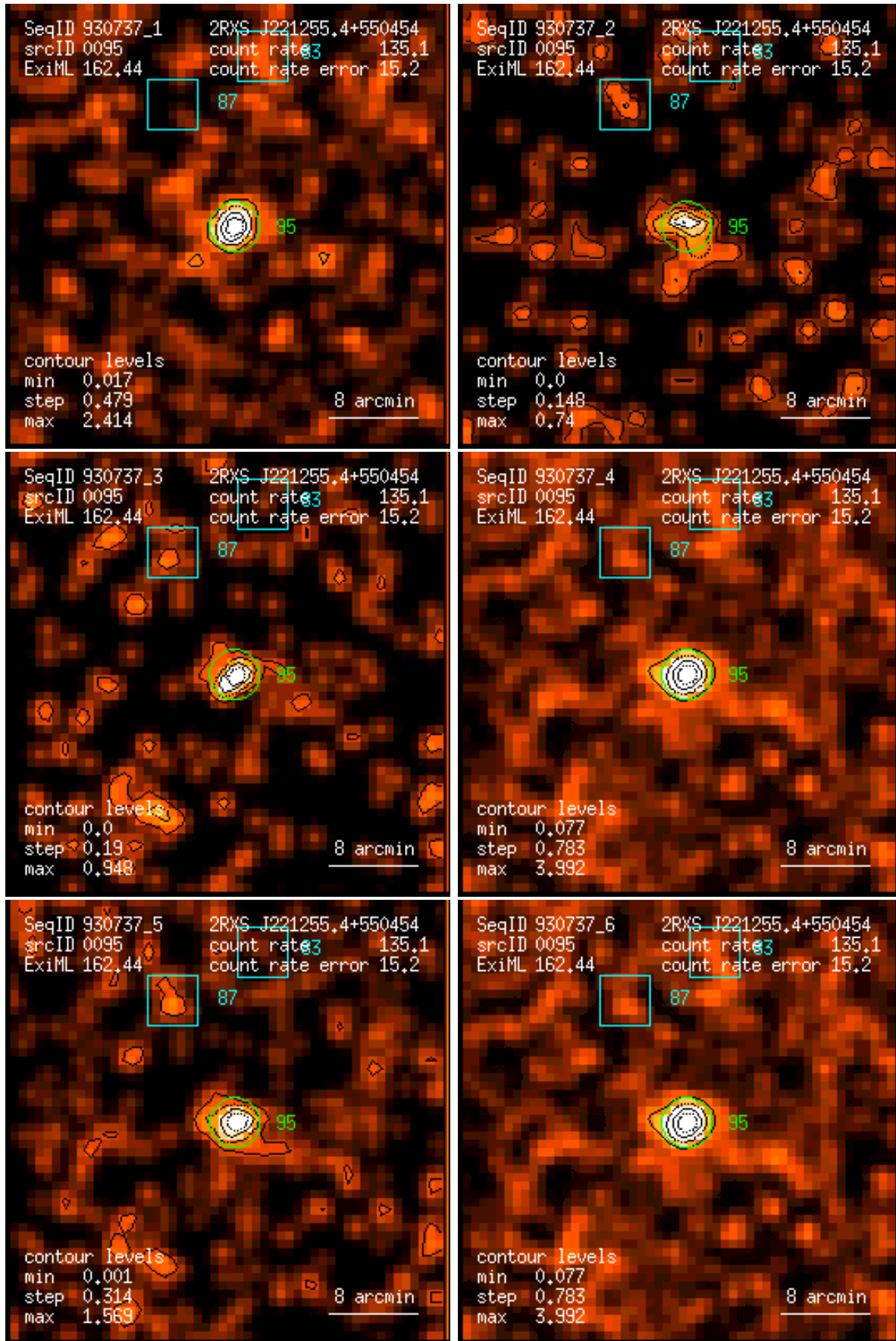
Figure 95: RASS 930737: detection 0095: band rate images, Gaussian filter: (1) PSPC channels 11 – 41, (2) 52 – 90, (3) 91 – 201, (4) 11 – 235, (5) 52 – 201, (6) 11 – 201. Broad band rates in counts/ks. Band rate contour levels in counts/ks/arcmin 2 .
