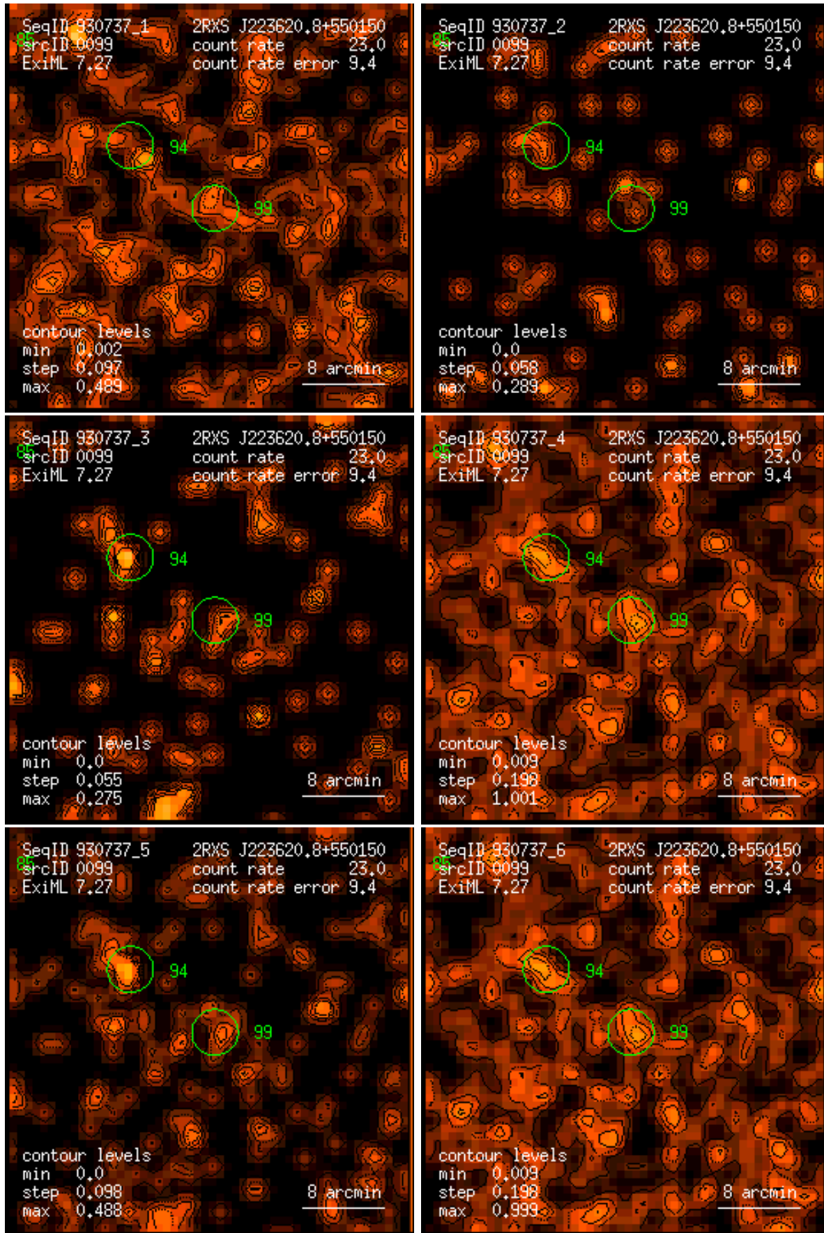
Figure 99: RASS 930737: detection 0099: band rate images, Gaussian filter: (1) PSPC channels 11 – 41, (2) 52 – 90, (3) 91 – 201, (4) 11 – 235, (5) 52 – 201, (6) 11 – 201. Broad band rates in counts/ks. Band rate contour levels in counts/ks/arcmin 2 .
