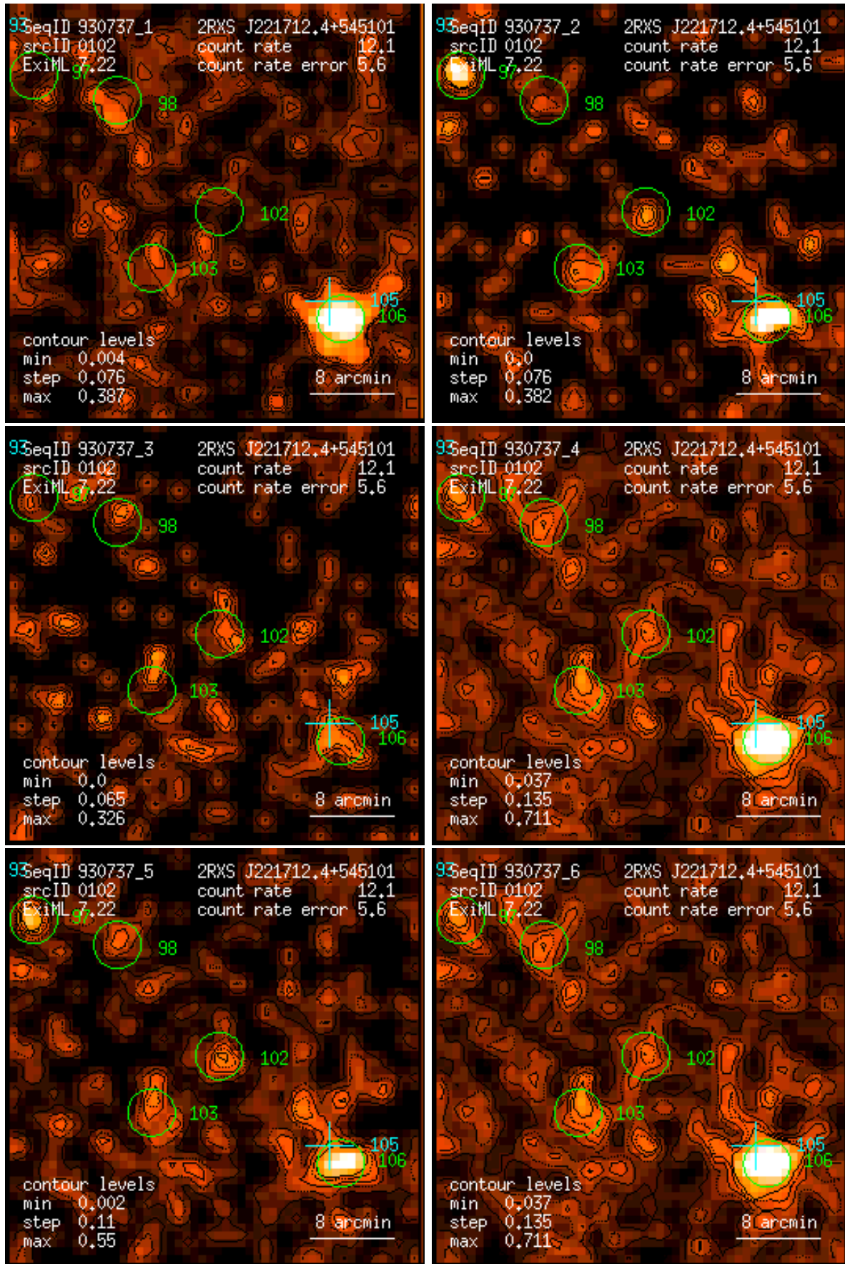
Figure 102: RASS 930737: detection 0102: band rate images, Gaussian filter: (1) PSPC channels 11 – 41, (2) 52 – 90, (3) 91 – 201, (4) 11 – 235, (5) 52 – 201, (6) 11 – 201. Broad band rates in counts/ks. Band rate contour levels in counts/ks/arcmin 2 .
