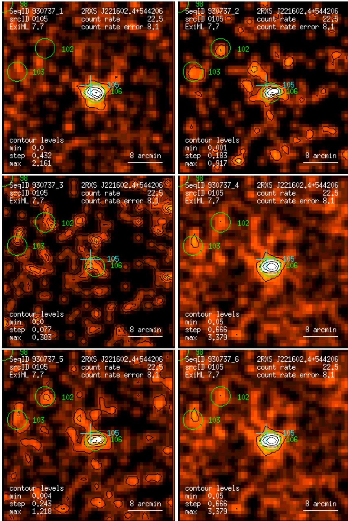
Figure 105: RASS 930737: detection 0105: band rate images, Gaussian filter: (1) PSPC channels 11 – 41, (2) 52 – 90, (3) 91 – 201, (4) 11 – 235, (5) 52 – 201, (6) 11 – 201. Broad band rates in counts/ks. Band rate contour levels in counts/ks/arcmin 2 .
