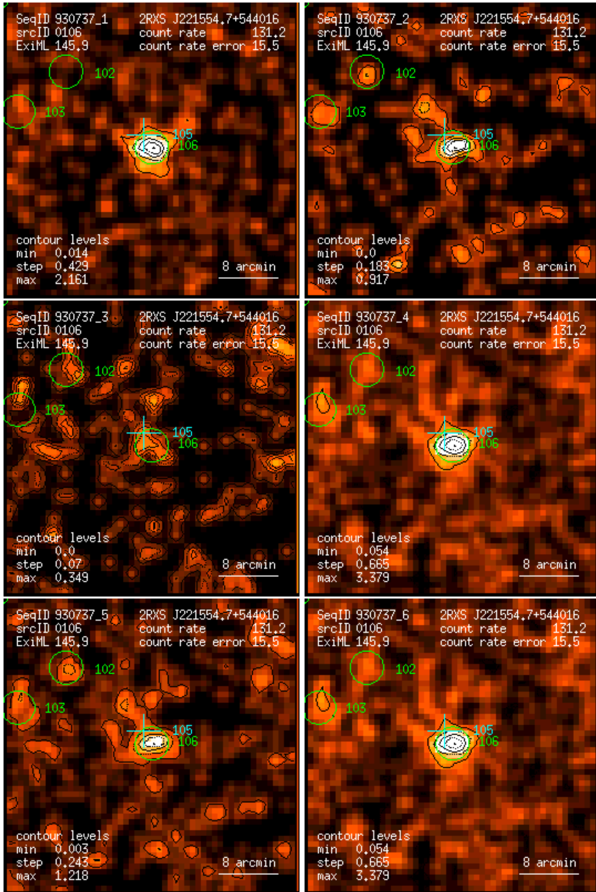
Figure 106: RASS 930737: detection 0106: band rate images, Gaussian filter: (1) PSPC channels 11 – 41, (2) 52 – 90, (3) 91 – 201, (4) 11 – 235, (5) 52 – 201, (6) 11 – 201. Broad band rates in counts/ks. Band rate contour levels in counts/ks/arcmin 2 .
