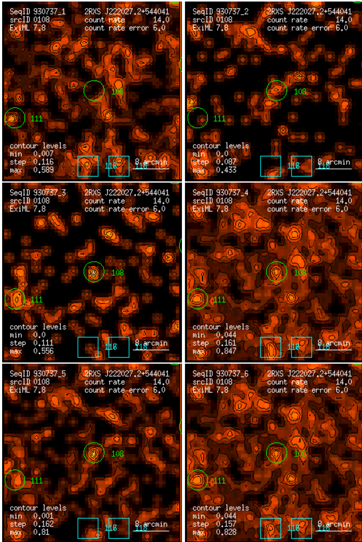
Figure 108: RASS 930737: detection 0108: band rate images, Gaussian filter: (1) PSPC channels 11 – 41, (2) 52 – 90, (3) 91 – 201, (4) 11 – 235, (5) 52 – 201, (6) 11 – 201. Broad band rates in counts/ks. Band rate contour levels in counts/ks/arcmin 2 .
