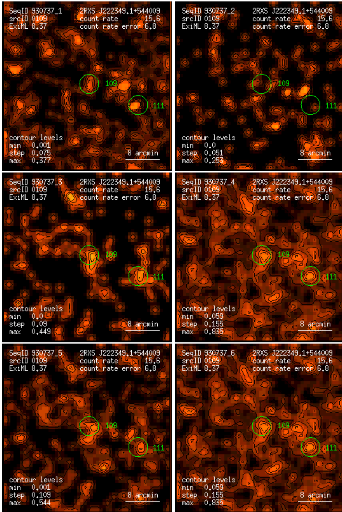
Figure 109: RASS 930737: detection 0109: band rate images, Gaussian filter: (1) PSPC channels 11 – 41, (2) 52 – 90, (3) 91 – 201, (4) 11 – 235, (5) 52 – 201, (6) 11 – 201. Broad band rates in counts/ks. Band rate contour levels in counts/ks/arcmin 2 .
