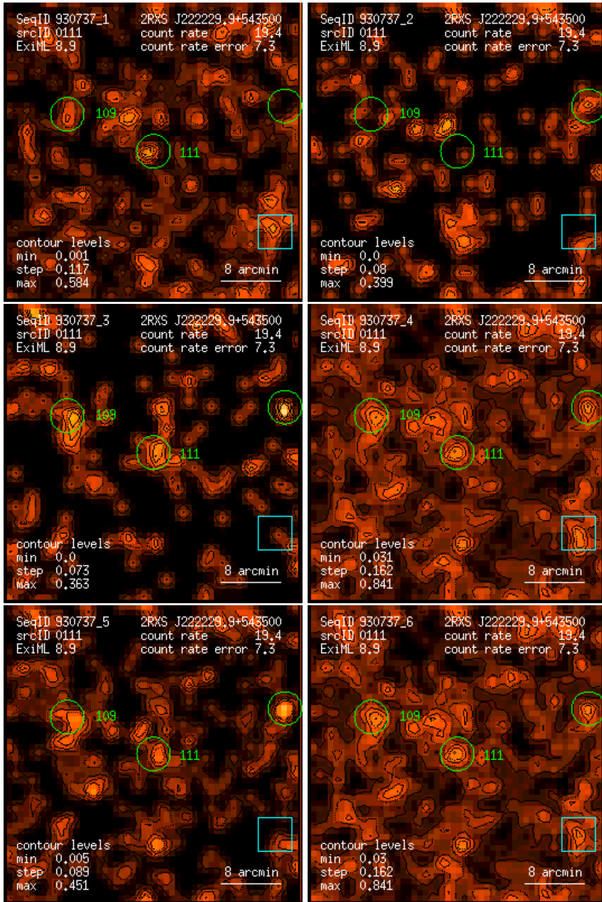
Figure 111: RASS 930737: detection 0111: band rate images, Gaussian filter: (1) PSPC channels 11 – 41, (2) 52 – 90, (3) 91 – 201, (4) 11 – 235, (5) 52 – 201, (6) 11 – 201. Broad band rates in counts/ks. Band rate contour levels in counts/ks/arcmin 2 .
