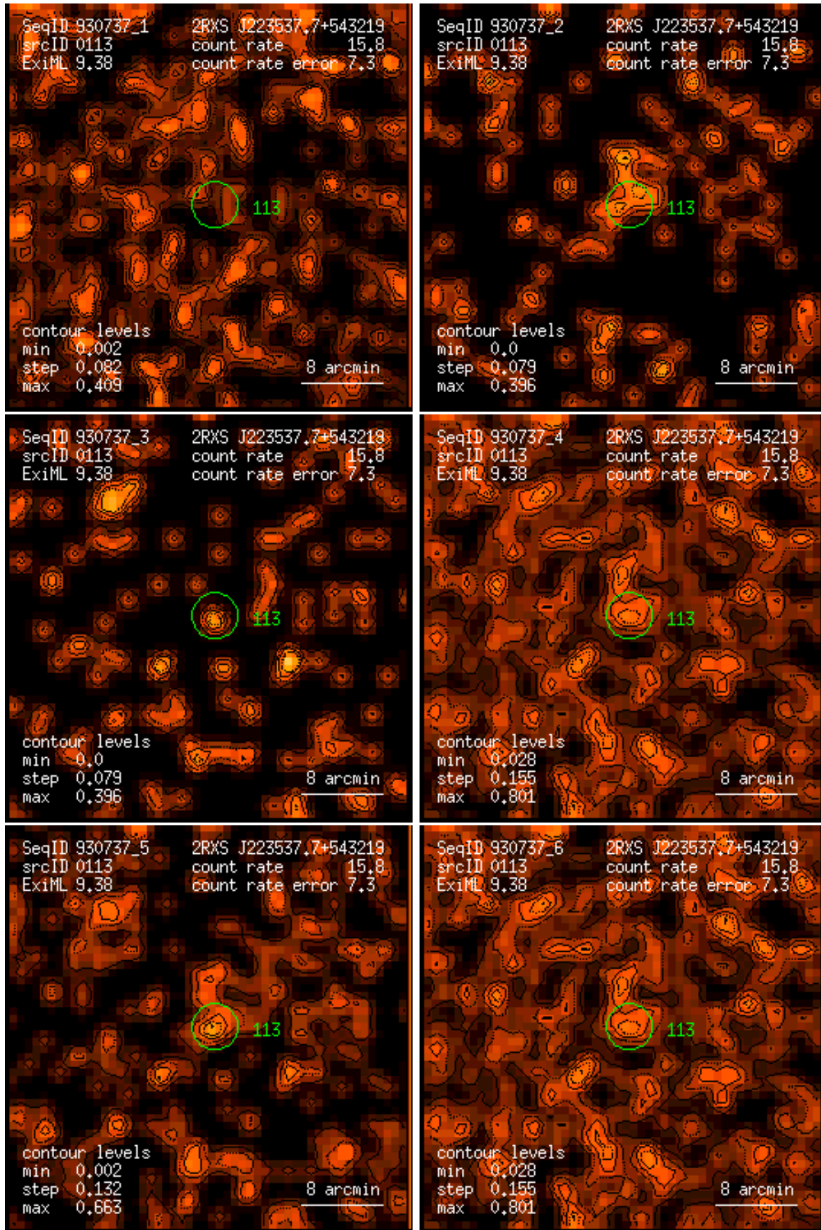
Figure 113: RASS 930737: detection 0113: band rate images, Gaussian filter: (1) PSPC channels 11 – 41, (2) 52 – 90, (3) 91 – 201, (4) 11 – 235, (5) 52 – 201, (6) 11 – 201. Broad band rates in counts/ks. Band rate contour levels in counts/ks/arcmin 2 .
