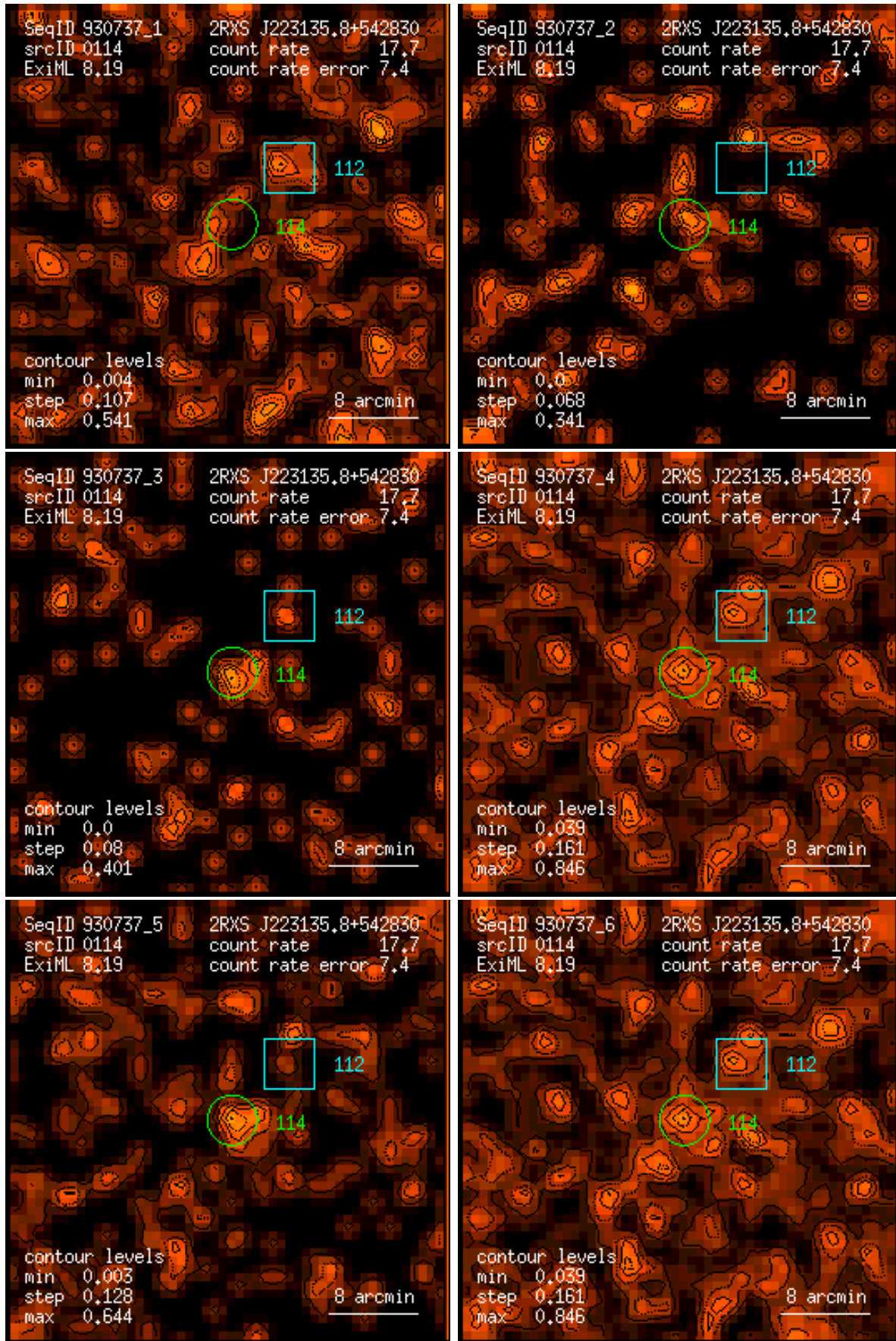
Figure 114: RASS 930737: detection 0114: band rate images, Gaussian filter: (1) PSPC channels 11 – 41, (2) 52 – 90, (3) 91 – 201, (4) 11 – 235, (5) 52 – 201, (6) 11 – 201. Broad band rates in counts/ks. Band rate contour levels in counts/ks/arcmin 2 .
