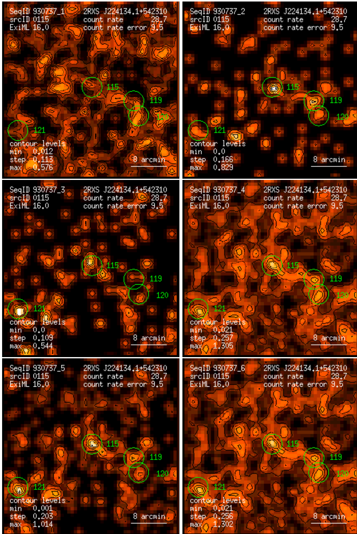
Figure 115: RASS 930737: detection 0115: band rate images, Gaussian filter: (1) PSPC channels 11 – 41, (2) 52 – 90, (3) 91 – 201, (4) 11 – 235, (5) 52 – 201, (6) 11 – 201. Broad band rates in counts/ks. Band rate contour levels in counts/ks/arcmin 2 .
