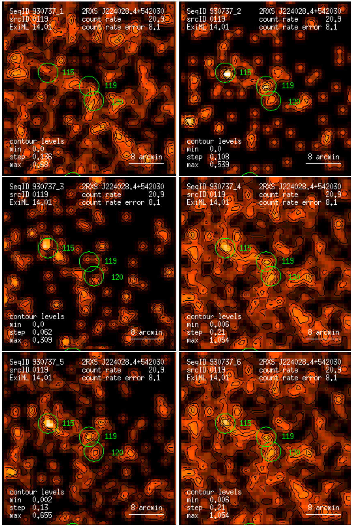
Figure 119: RASS 930737: detection 0119: band rate images, Gaussian filter: (1) PSPC channels 11 – 41, (2) 52 – 90, (3) 91 – 201, (4) 11 – 235, (5) 52 – 201, (6) 11 – 201. Broad band rates in counts/ks. Band rate contour levels in counts/ks/arcmin 2 .
