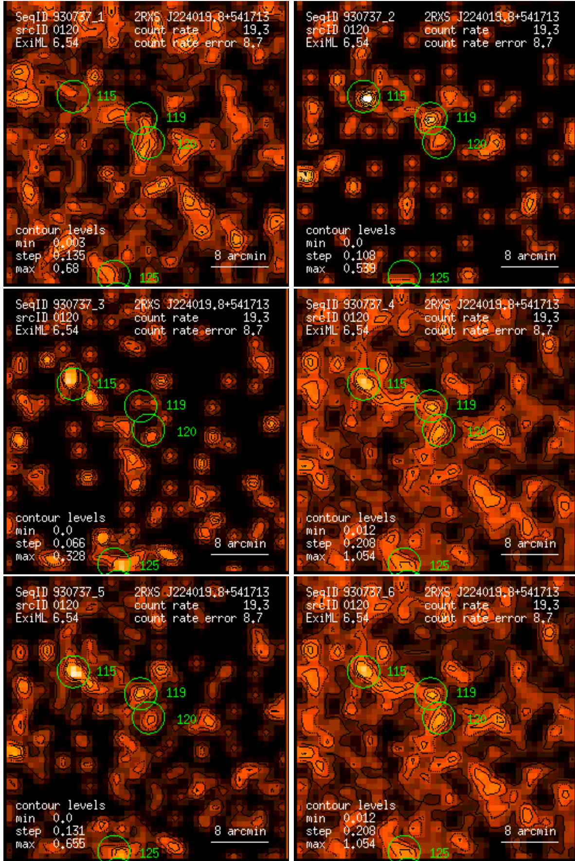
Figure 120: RASS 930737: detection 0120: band rate images, Gaussian filter: (1) PSPC channels 11 – 41, (2) 52 – 90, (3) 91 – 201, (4) 11 – 235, (5) 52 – 201, (6) 11 – 201. Broad band rates in counts/ks. Band rate contour levels in counts/ks/arcmin 2 .
