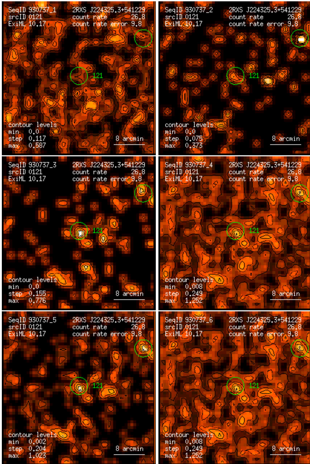
Figure 121: RASS 930737: detection 0121: band rate images, Gaussian filter: (1) PSPC channels 11 – 41, (2) 52 – 90, (3) 91 – 201, (4) 11 – 235, (5) 52 – 201, (6) 11 – 201. Broad band rates in counts/ks. Band rate contour levels in counts/ks/arcmin 2 .
