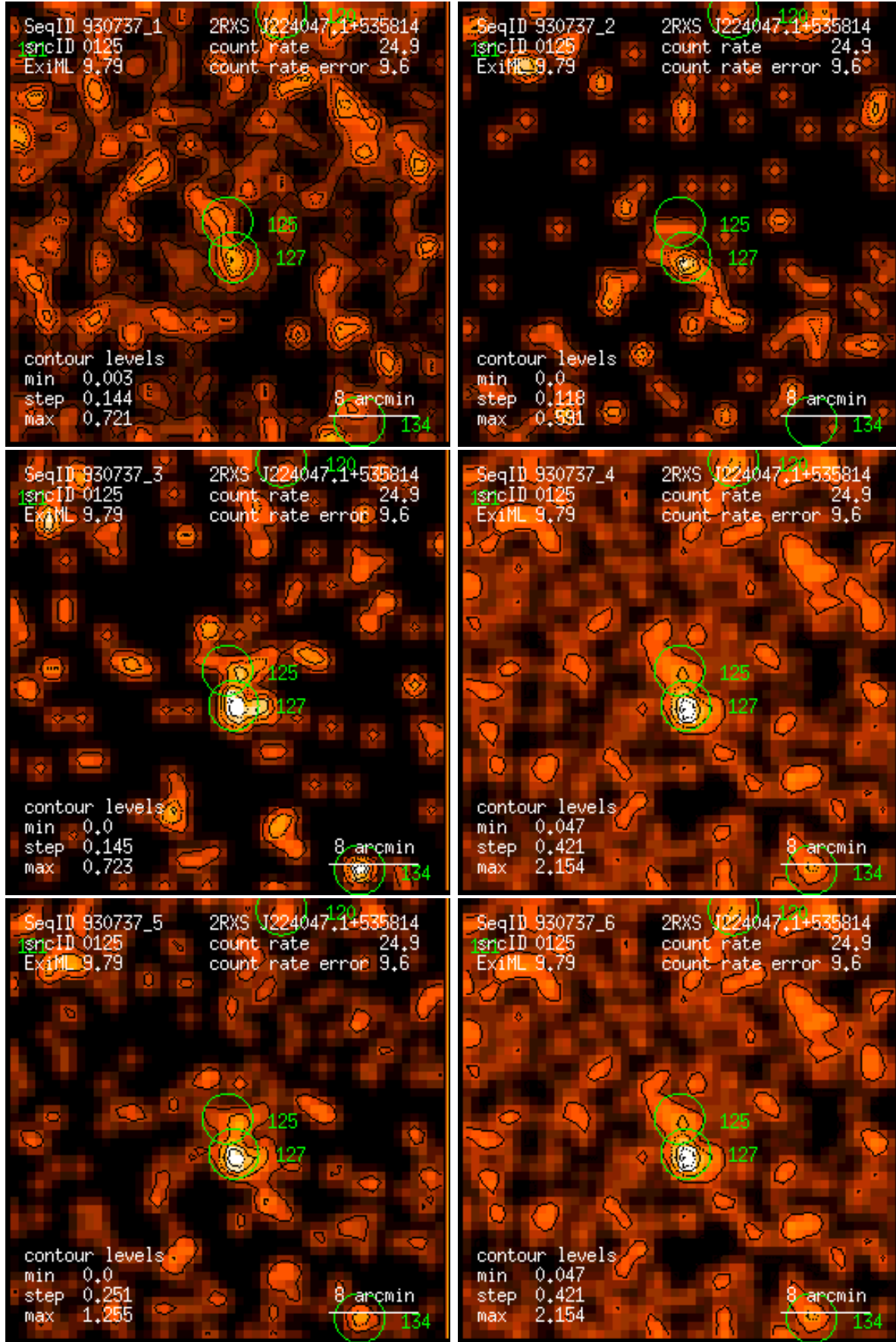
Figure 125: RASS 930737: detection 0125: band rate images, Gaussian filter: (1) PSPC channels 11 – 41, (2) 52 – 90, (3) 91 – 201, (4) 11 – 235, (5) 52 – 201, (6) 11 – 201. Broad band rates in counts/ks. Band rate contour levels in counts/ks/arcmin 2 .
