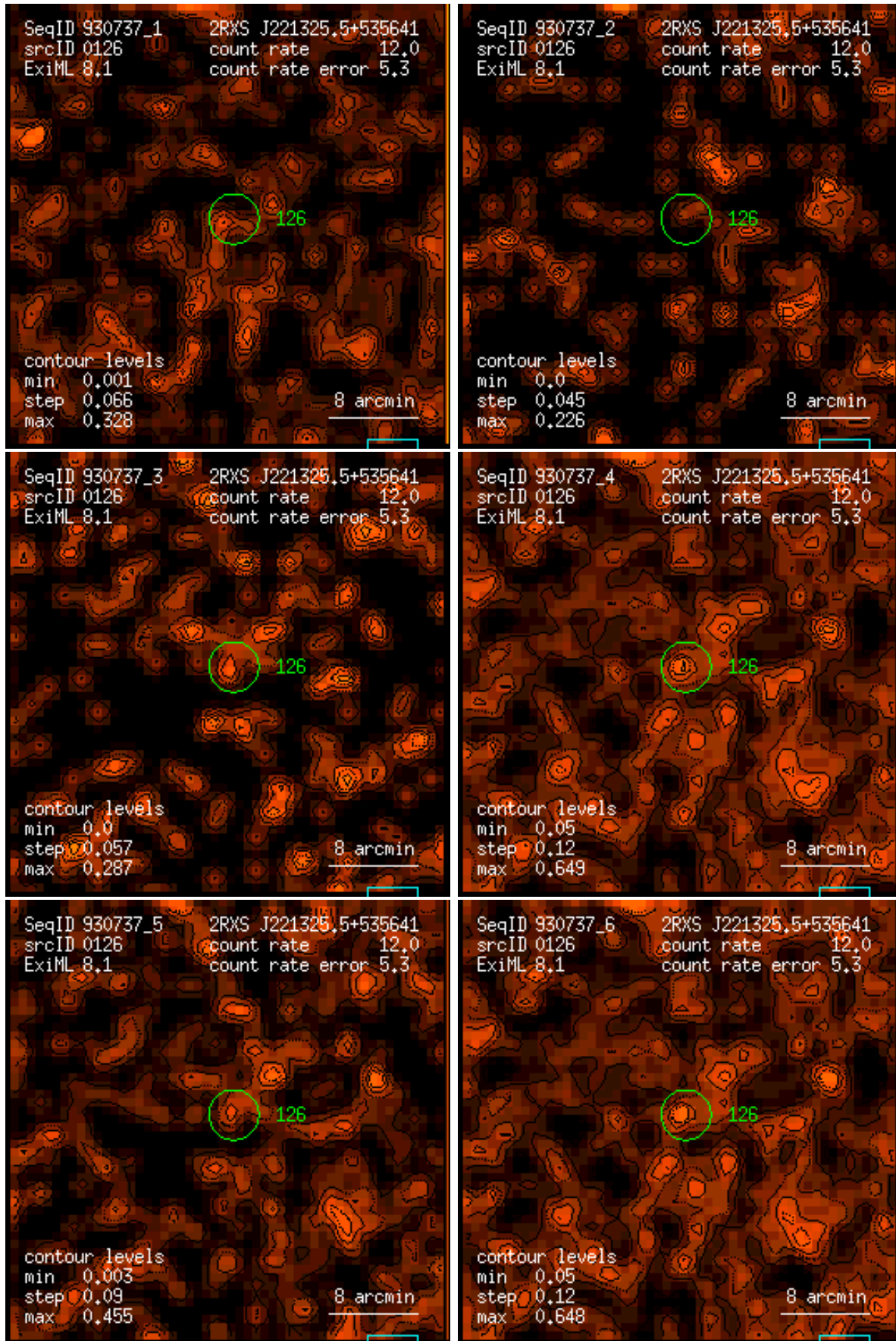
Figure 126: RASS 930737: detection 0126: band rate images, Gaussian filter: (1) PSPC channels 11 – 41, (2) 52 – 90, (3) 91 – 201, (4) 11 – 235, (5) 52 – 201, (6) 11 – 201. Broad band rates in counts/ks. Band rate contour levels in counts/ks/arcmin 2 .
