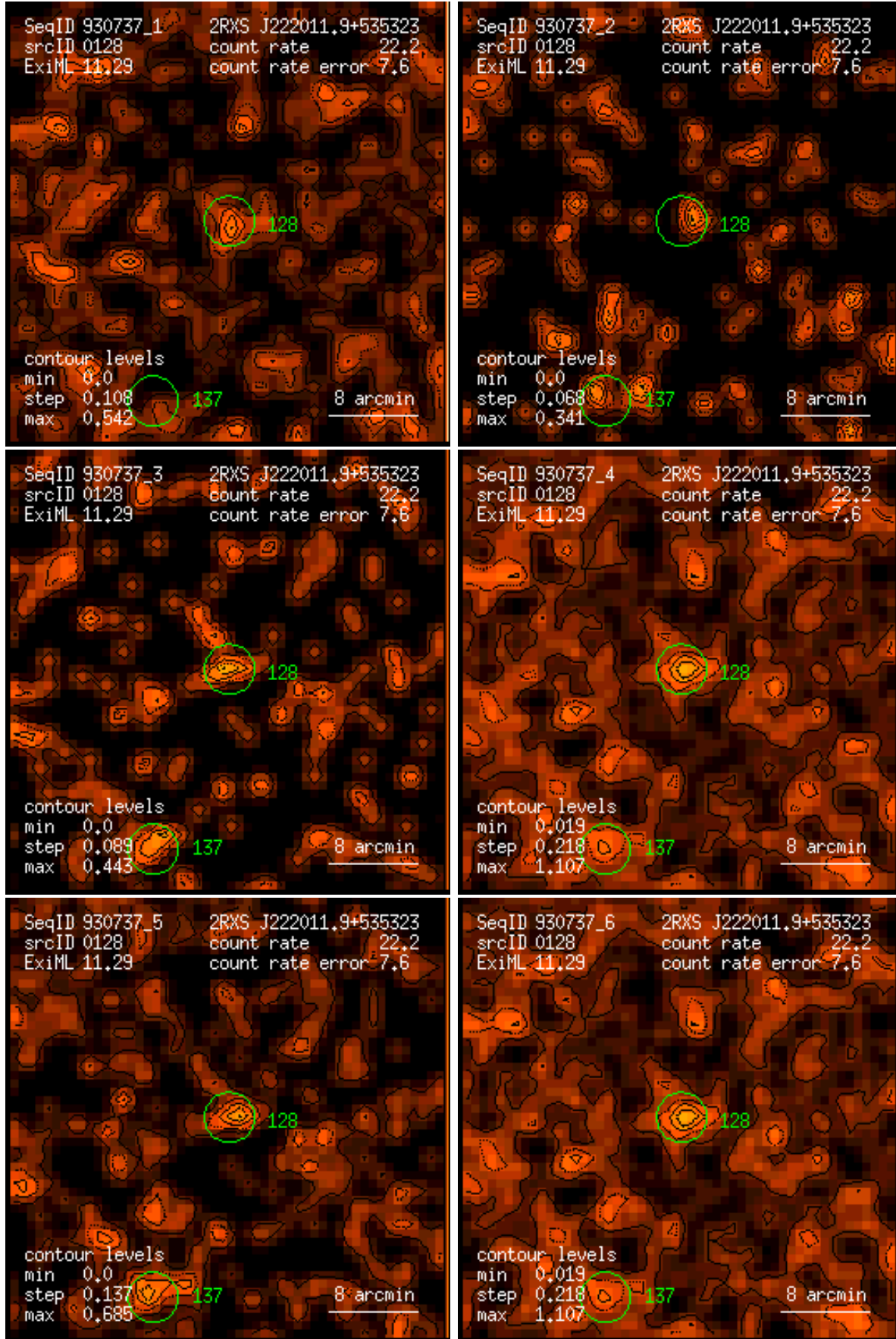
Figure 128: RASS 930737: detection 0128: band rate images, Gaussian filter: (1) PSPC channels 11 – 41, (2) 52 – 90, (3) 91 – 201, (4) 11 – 235, (5) 52 – 201, (6) 11 – 201. Broad band rates in counts/ks. Band rate contour levels in counts/ks/arcmin 2 .
