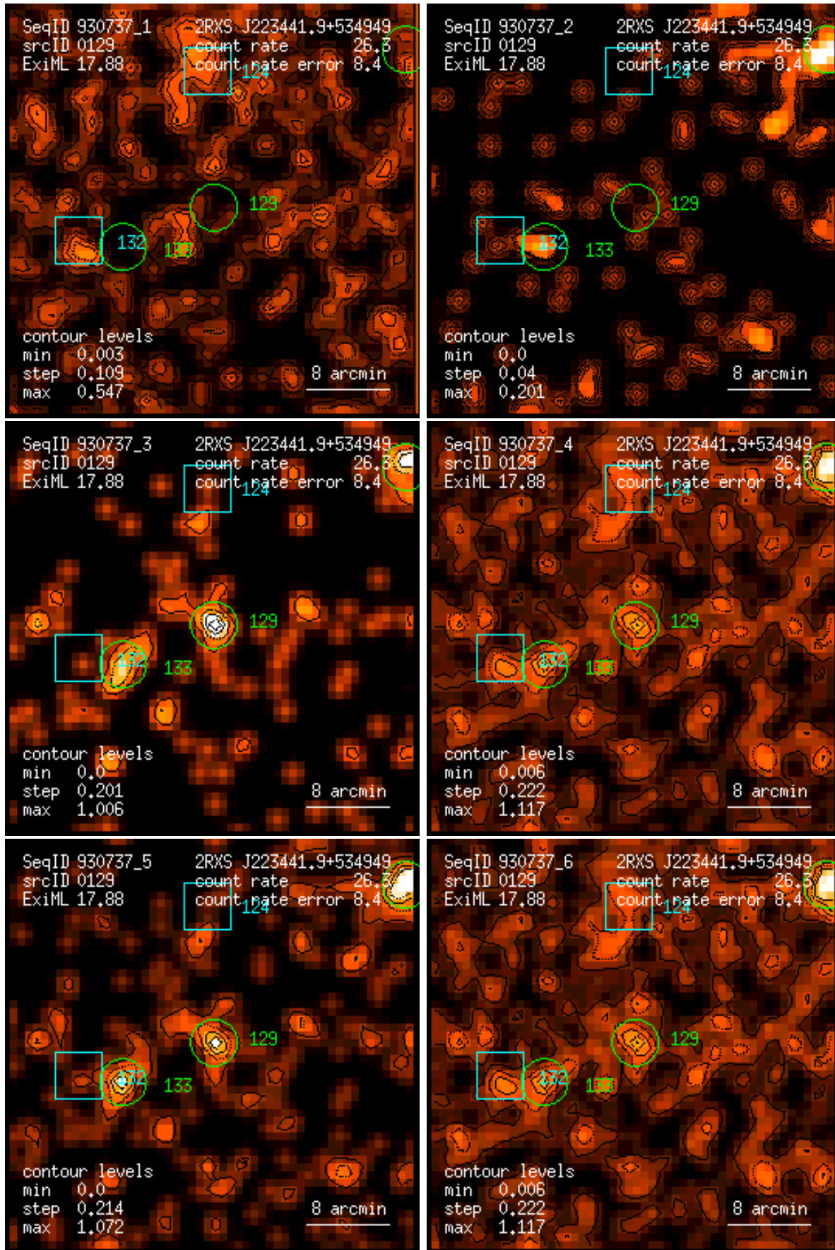
Figure 129: RASS 930737: detection 0129: band rate images, Gaussian filter: (1) PSPC channels 11 – 41, (2) 52 – 90, (3) 91 – 201, (4) 11 – 235, (5) 52 – 201, (6) 11 – 201. Broad band rates in counts/ks. Band rate contour levels in counts/ks/arcmin 2 .
