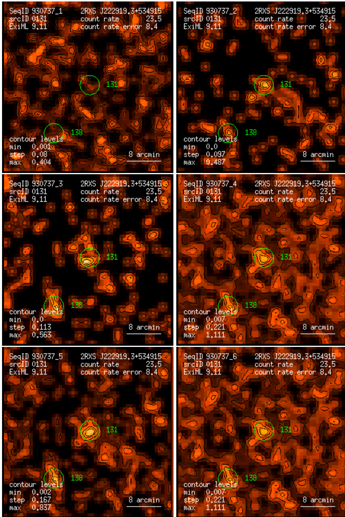
Figure 131: RASS 930737: detection 0131: band rate images, Gaussian filter: (1) PSPC channels 11 – 41, (2) 52 – 90, (3) 91 – 201, (4) 11 – 235, (5) 52 – 201, (6) 11 – 201. Broad band rates in counts/ks. Band rate contour levels in counts/ks/arcmin 2 .
