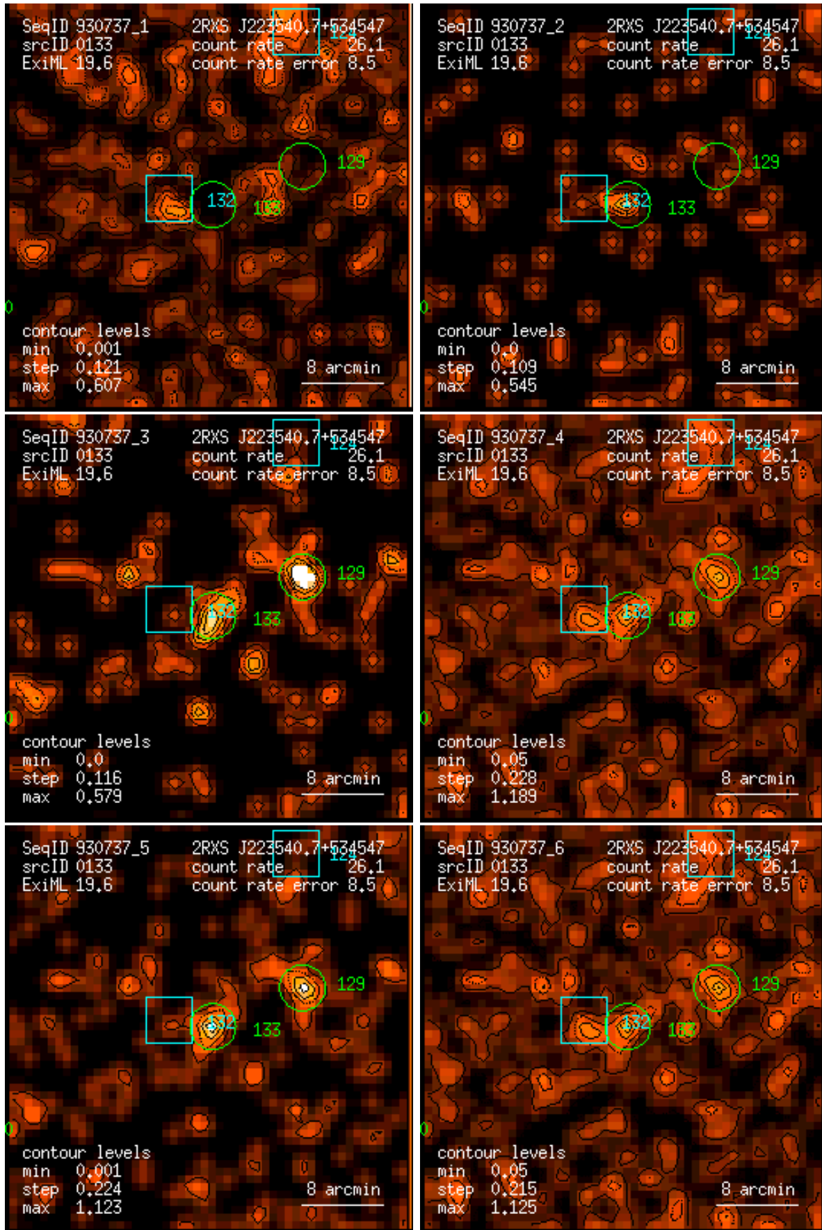
Figure 133: RASS 930737: detection 0133: band rate images, Gaussian filter: (1) PSPC channels 11 – 41, (2) 52 – 90, (3) 91 – 201, (4) 11 – 235, (5) 52 – 201, (6) 11 – 201. Broad band rates in counts/ks. Band rate contour levels in counts/ks/arcmin 2 .
