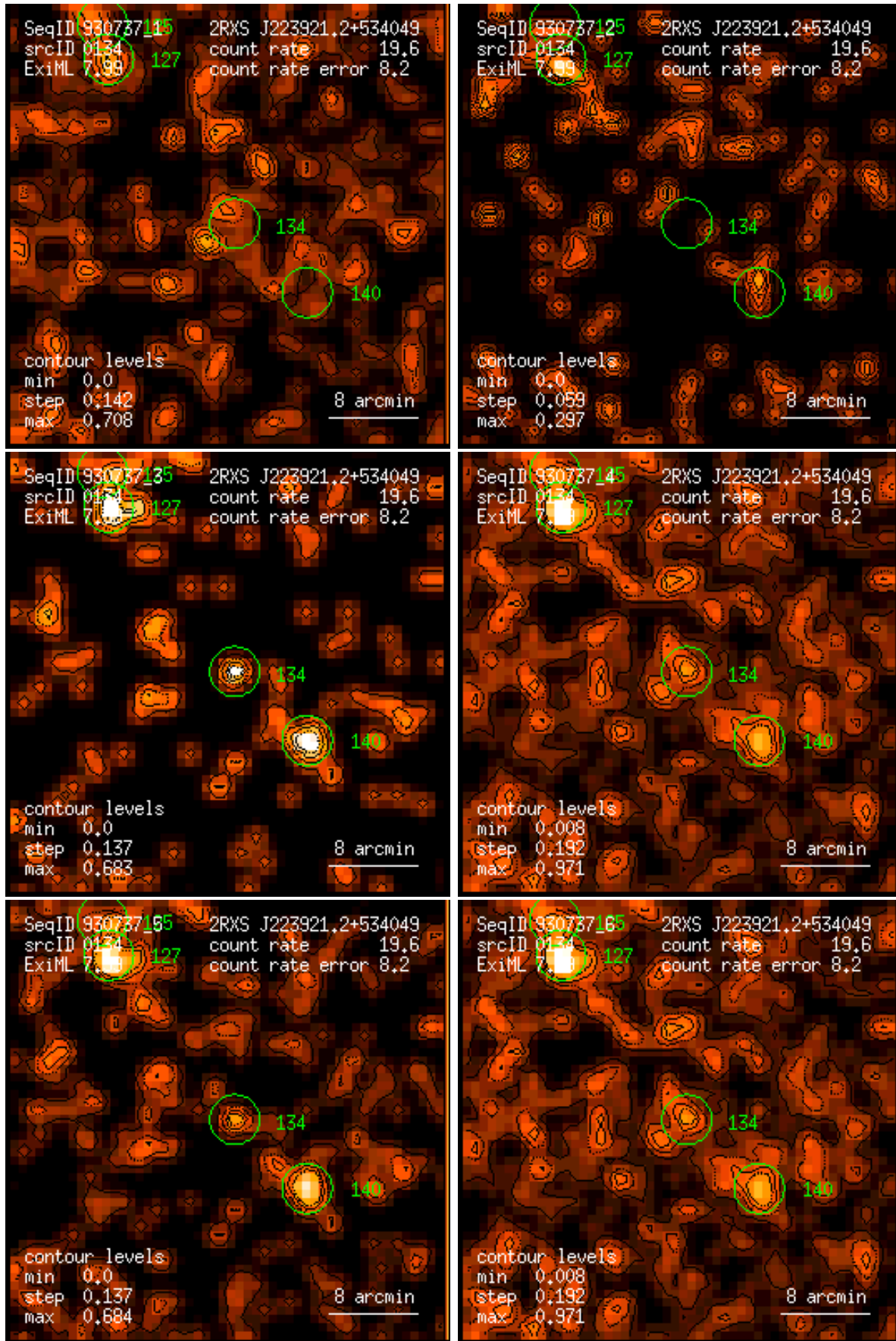
Figure 134: RASS 930737: detection 0134: band rate images, Gaussian filter: (1) PSPC channels 11 – 41, (2) 52 – 90, (3) 91 – 201, (4) 11 – 235, (5) 52 – 201, (6) 11 – 201. Broad band rates in counts/ks. Band rate contour levels in counts/ks/arcmin 2 .
