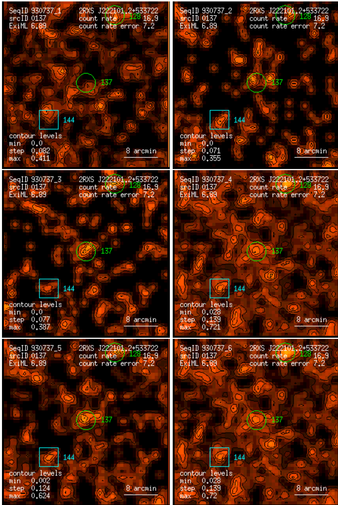
Figure 137: RASS 930737: detection 0137: band rate images, Gaussian filter: (1) PSPC channels 11 – 41, (2) 52 – 90, (3) 91 – 201, (4) 11 – 235, (5) 52 – 201, (6) 11 – 201. Broad band rates in counts/ks. Band rate contour levels in counts/ks/arcmin 2 .
