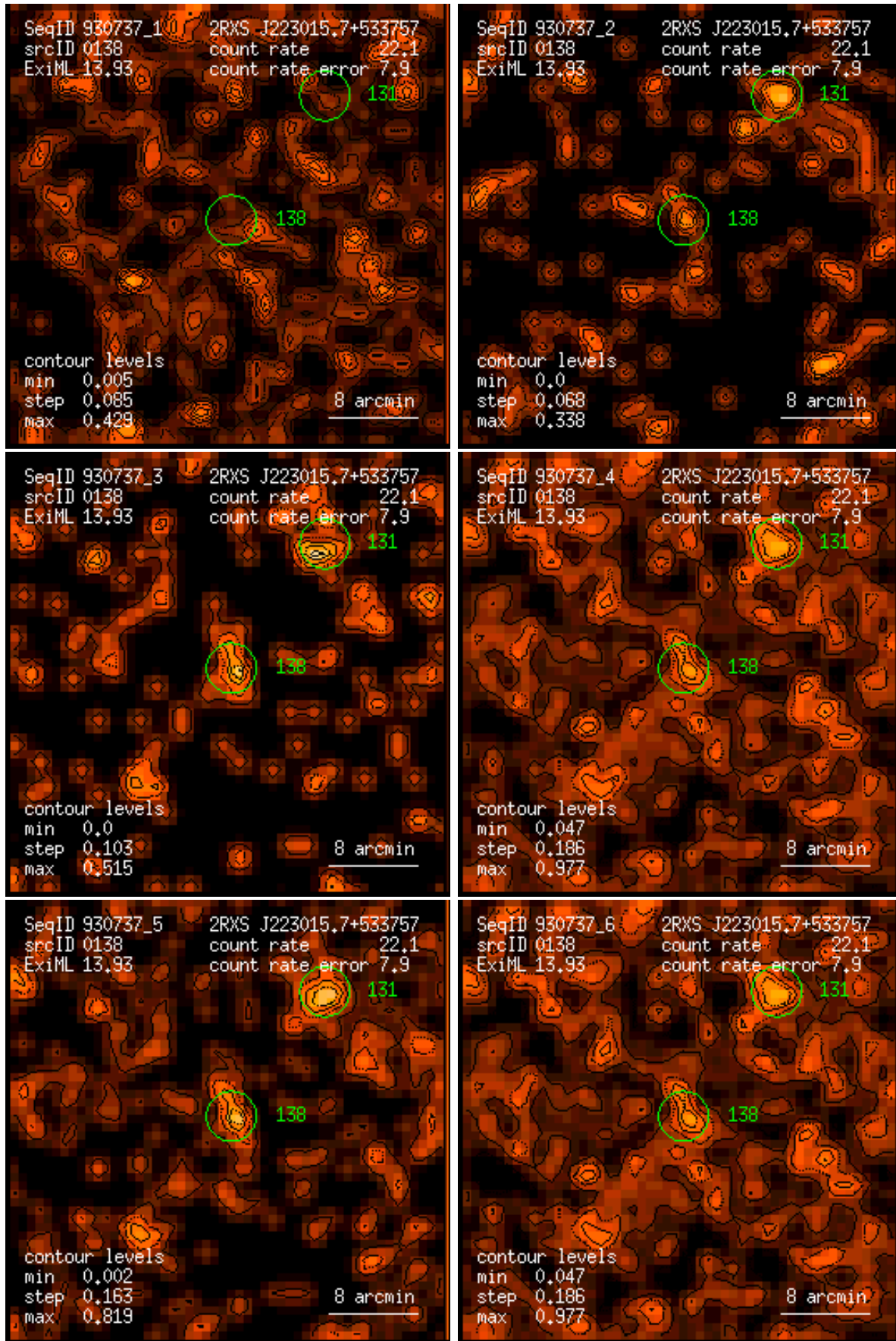
Figure 138: RASS 930737: detection 0138: band rate images, Gaussian filter: (1) PSPC channels 11 – 41, (2) 52 – 90, (3) 91 – 201, (4) 11 – 235, (5) 52 – 201, (6) 11 – 201. Broad band rates in counts/ks. Band rate contour levels in counts/ks/arcmin 2 .
