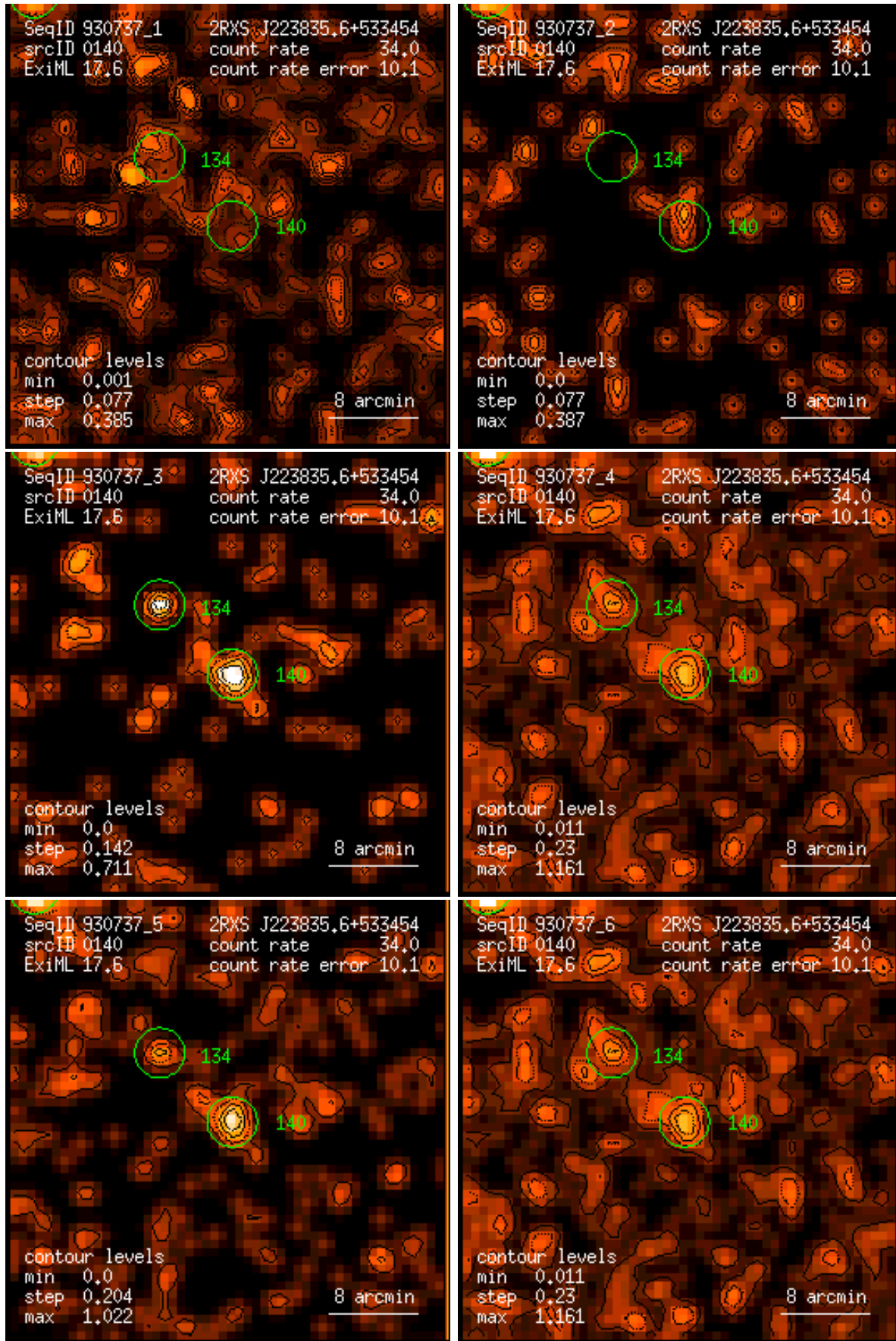
Figure 140: RASS 930737: detection 0140: band rate images, Gaussian filter: (1) PSPC channels 11 – 41, (2) 52 – 90, (3) 91 – 201, (4) 11 – 235, (5) 52 – 201, (6) 11 – 201. Broad band rates in counts/ks. Band rate contour levels in counts/ks/arcmin 2 .
