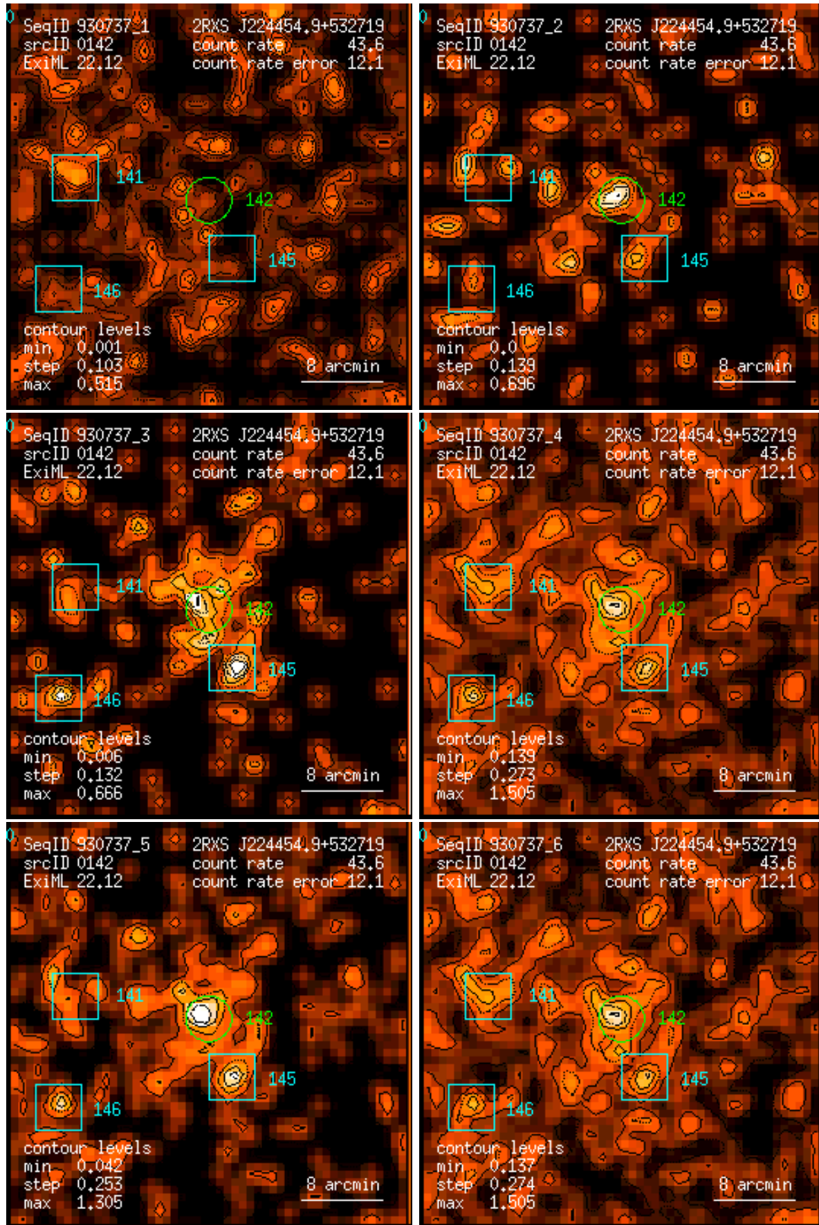
Figure 142: RASS 930737: detection 0142: band rate images, Gaussian filter: (1) PSPC channels 11 – 41, (2) 52 – 90, (3) 91 – 201, (4) 11 – 235, (5) 52 – 201, (6) 11 – 201. Broad band rates in counts/ks. Band rate contour levels in counts/ks/arcmin 2 .
