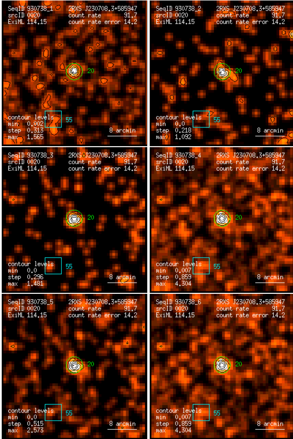
Figure 20: RASS 930738: detection 0020: band rate images, Gaussian filter: (1) PSPC channels 11 – 41, (2) 52 – 90, (3) 91 – 201, (4) 11 – 235, (5) 52 – 201, (6) 11 – 201. Broad band rates in counts/ks. Band rate contour levels in counts/ks/arcmin 2 .
