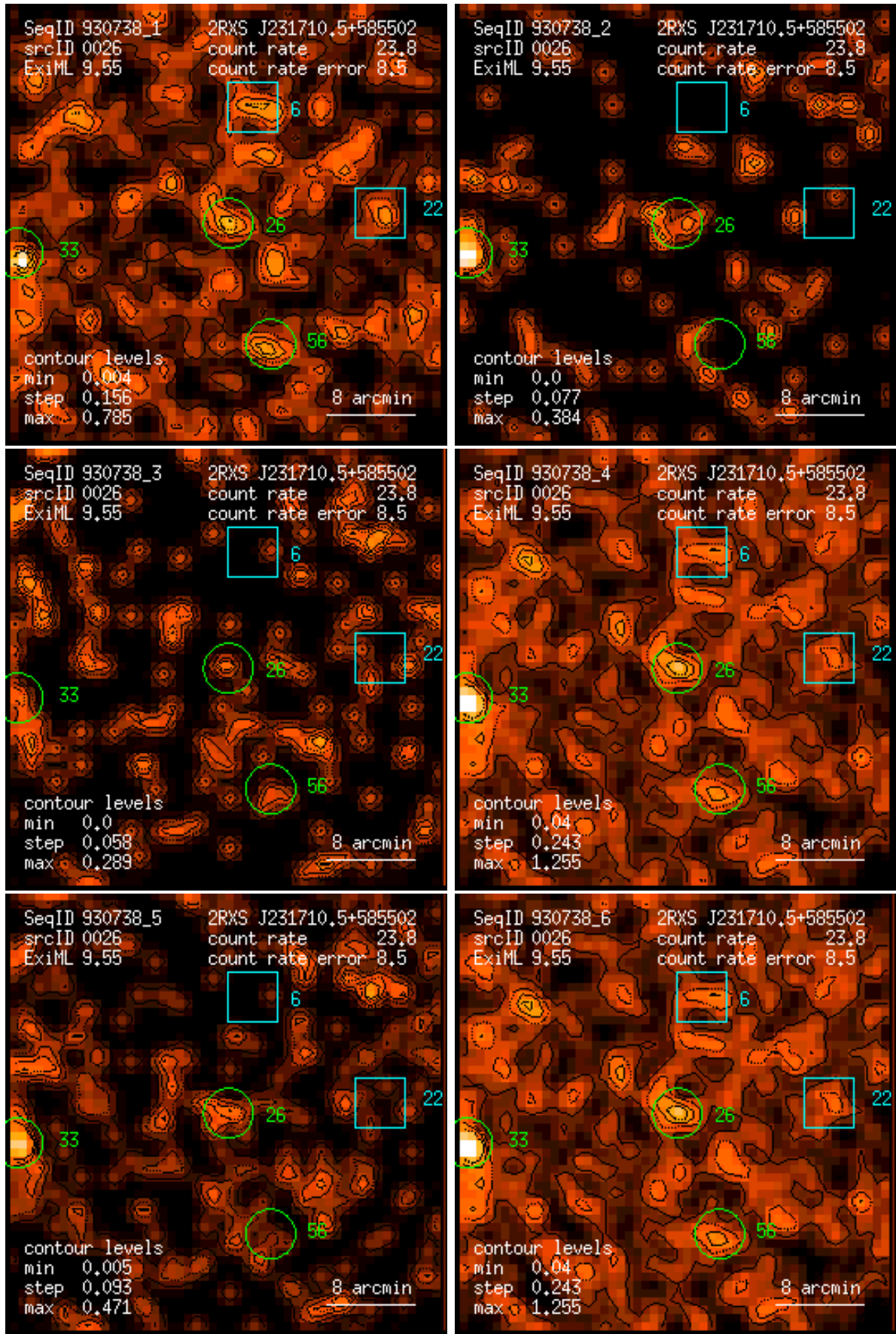
Figure 26: RASS 930738: detection 0026: band rate images, Gaussian filter: (1) PSPC channels 11 – 41, (2) 52 – 90, (3) 91 – 201, (4) 11 – 235, (5) 52 – 201, (6) 11 – 201. Broad band rates in counts/ks. Band rate contour levels in counts/ks/arcmin 2 .
