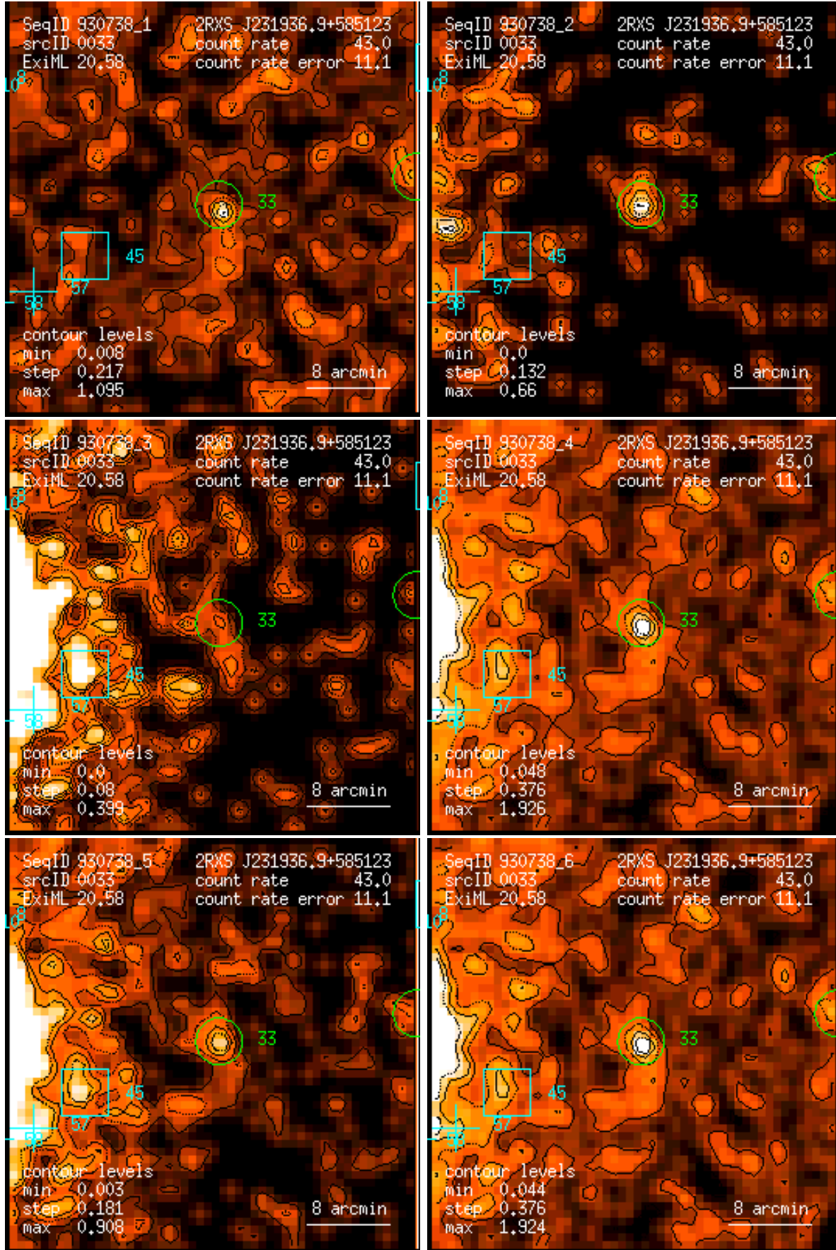
Figure 33: RASS 930738: detection 0033: band rate images, Gaussian filter: (1) PSPC channels 11 – 41, (2) 52 – 90, (3) 91 – 201, (4) 11 – 235, (5) 52 – 201, (6) 11 – 201. Broad band rates in counts/ks. Band rate contour levels in counts/ks/arcmin 2 .
