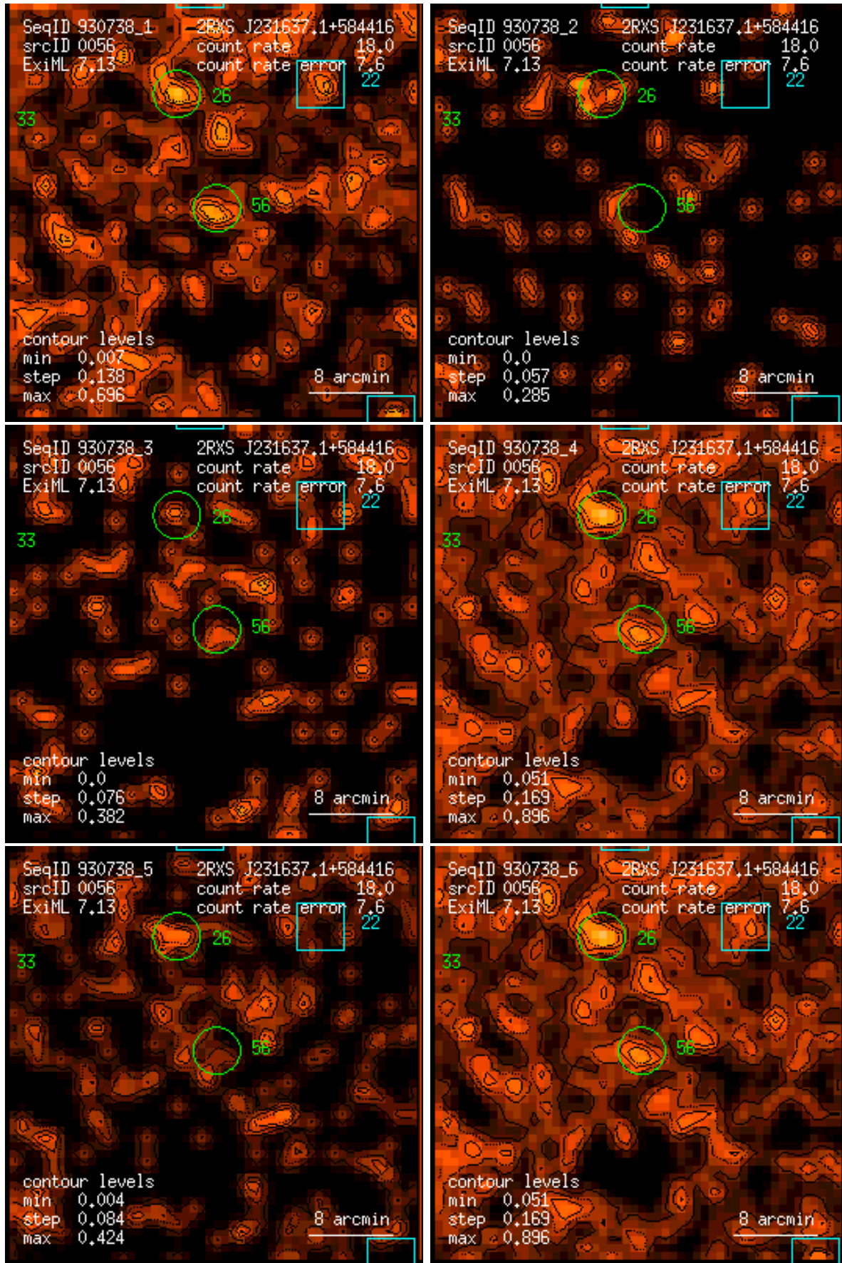
Figure 56: RASS 930738: detection 0056: band rate images, Gaussian filter: (1) PSPC channels 11 – 41, (2) 52 – 90, (3) 91 – 201, (4) 11 – 235, (5) 52 – 201, (6) 11 – 201. Broad band rates in counts/ks. Band rate contour levels in counts/ks/arcmin 2 .
