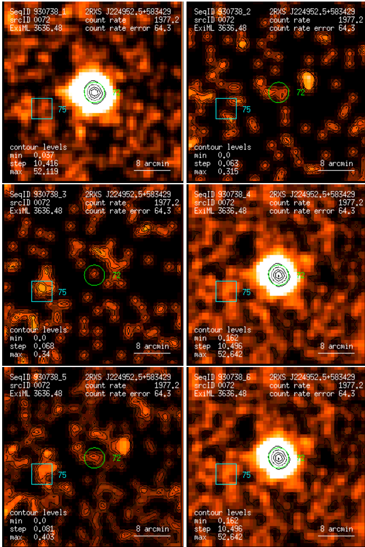
Figure 72: RASS 930738: detection 0072: band rate images, Gaussian filter: (1) PSPC channels 11 – 41, (2) 52 – 90, (3) 91 – 201, (4) 11 – 235, (5) 52 – 201, (6) 11 – 201. Broad band rates in counts/ks. Band rate contour levels in counts/ks/arcmin 2 .
