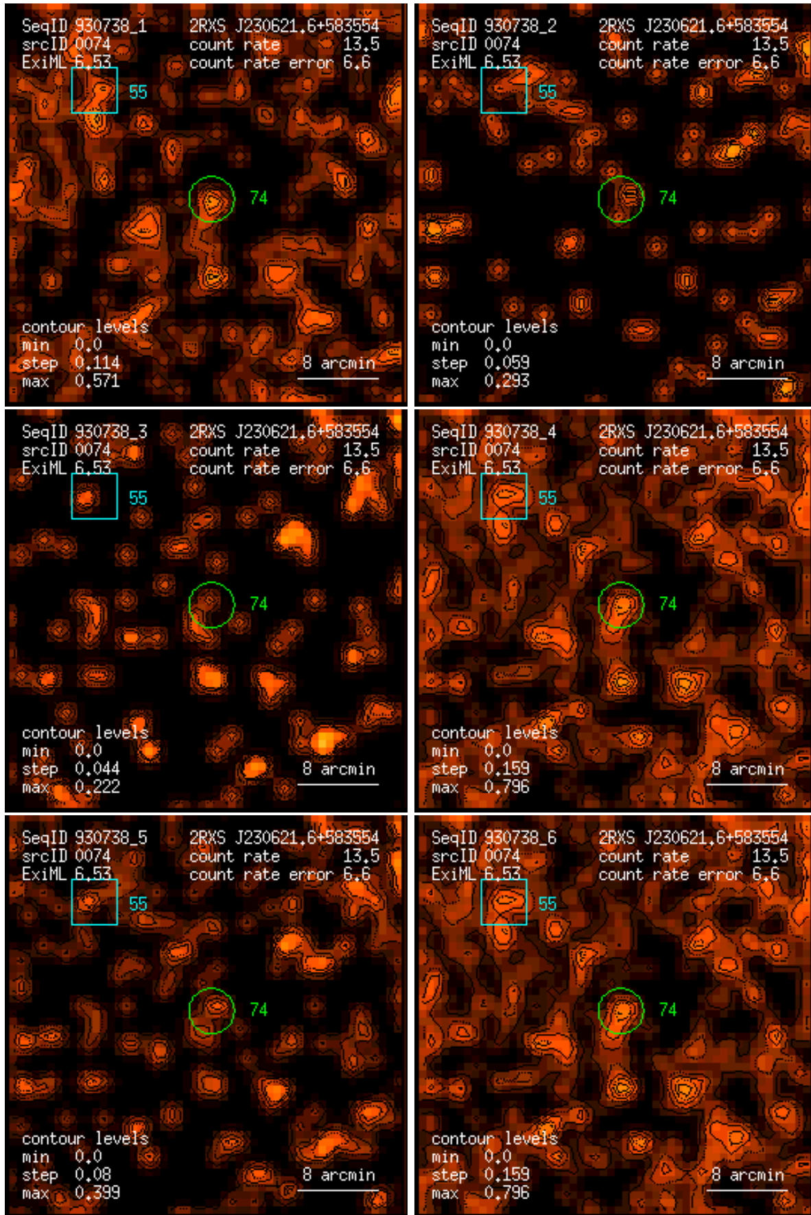
Figure 74: RASS 930738: detection 0074: band rate images, Gaussian filter: (1) PSPC channels 11 – 41, (2) 52 – 90, (3) 91 – 201, (4) 11 – 235, (5) 52 – 201, (6) 11 – 201. Broad band rates in counts/ks. Band rate contour levels in counts/ks/arcmin 2 .
