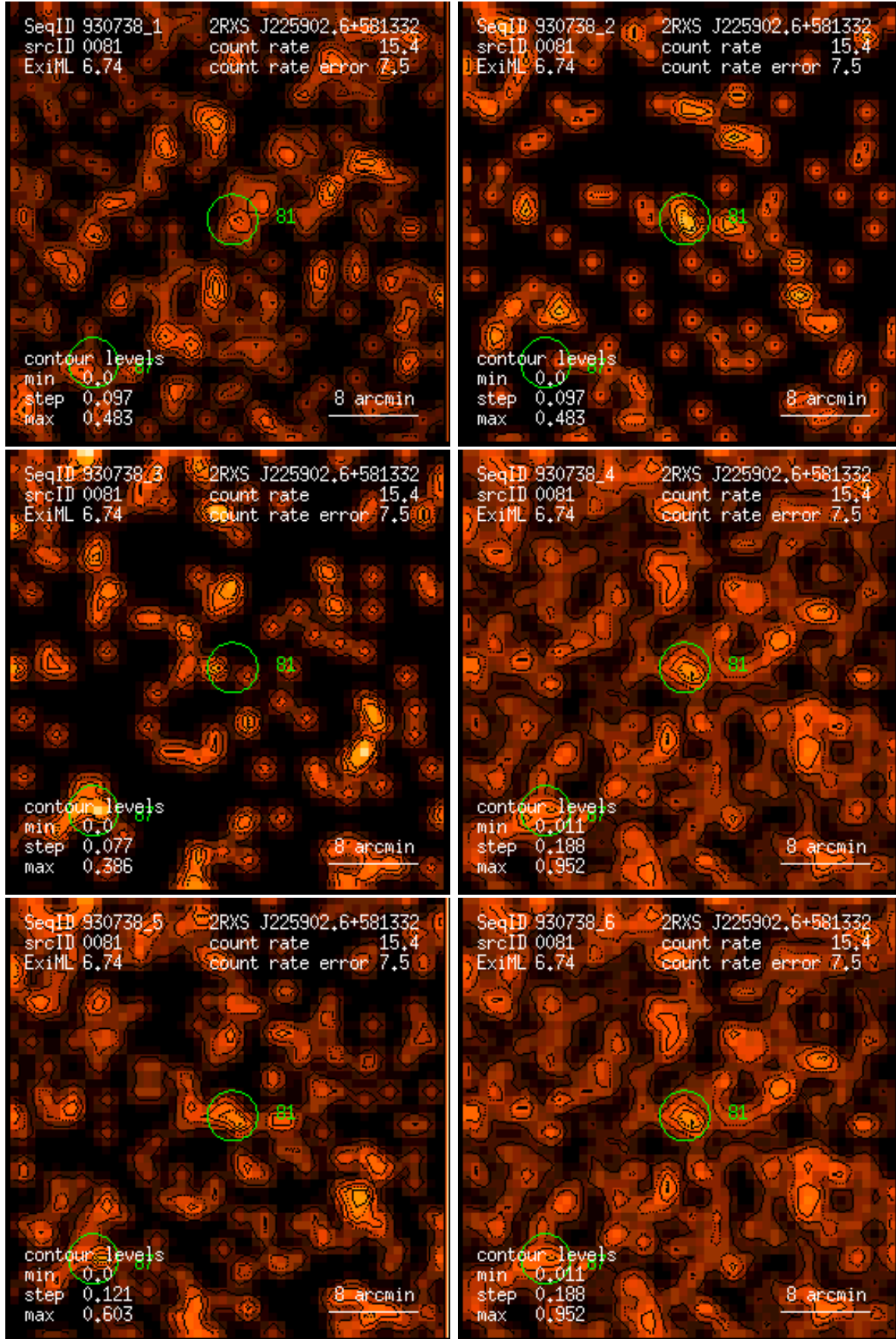
Figure 81: RASS 930738: detection 0081: band rate images, Gaussian filter: (1) PSPC channels 11 – 41, (2) 52 – 90, (3) 91 – 201, (4) 11 – 235, (5) 52 – 201, (6) 11 – 201. Broad band rates in counts/ks. Band rate contour levels in counts/ks/arcmin 2 .
