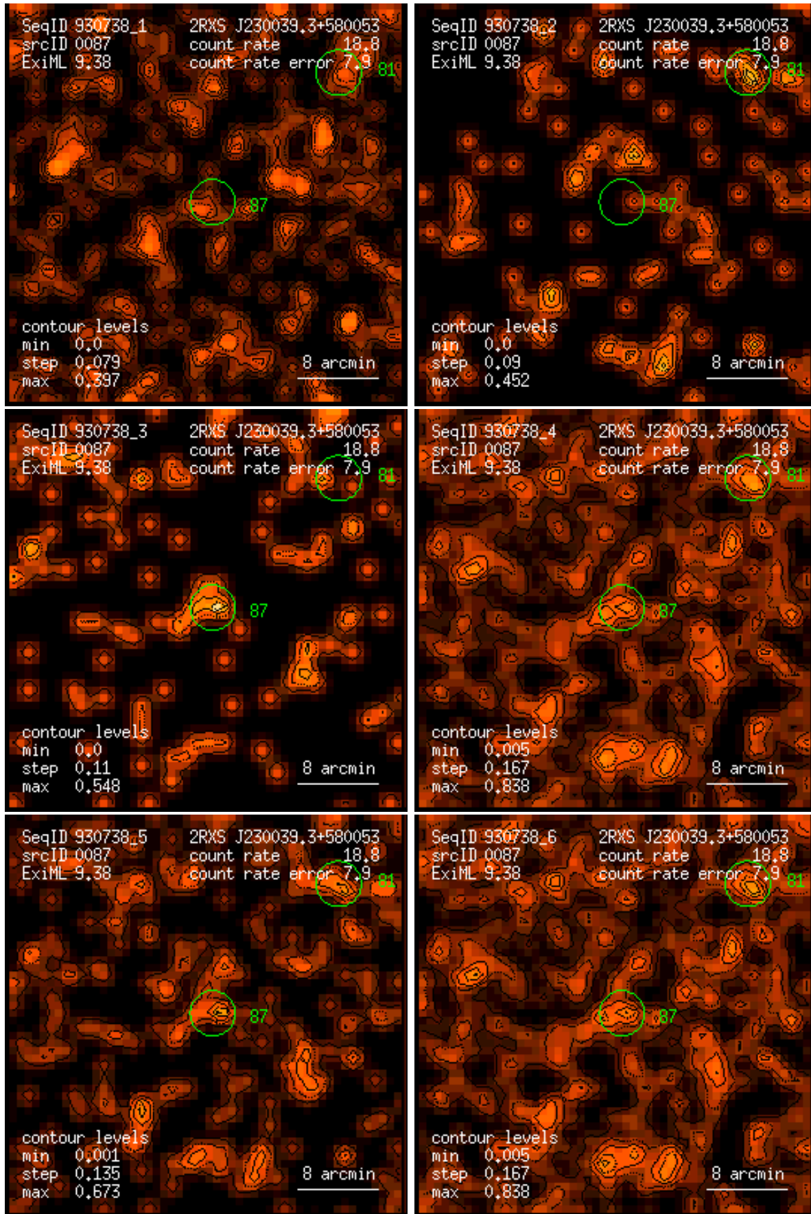
Figure 87: RASS 930738: detection 0087: band rate images, Gaussian filter: (1) PSPC channels 11 – 41, (2) 52 – 90, (3) 91 – 201, (4) 11 – 235, (5) 52 – 201, (6) 11 – 201. Broad band rates in counts/ks. Band rate contour levels in counts/ks/arcmin 2 .
