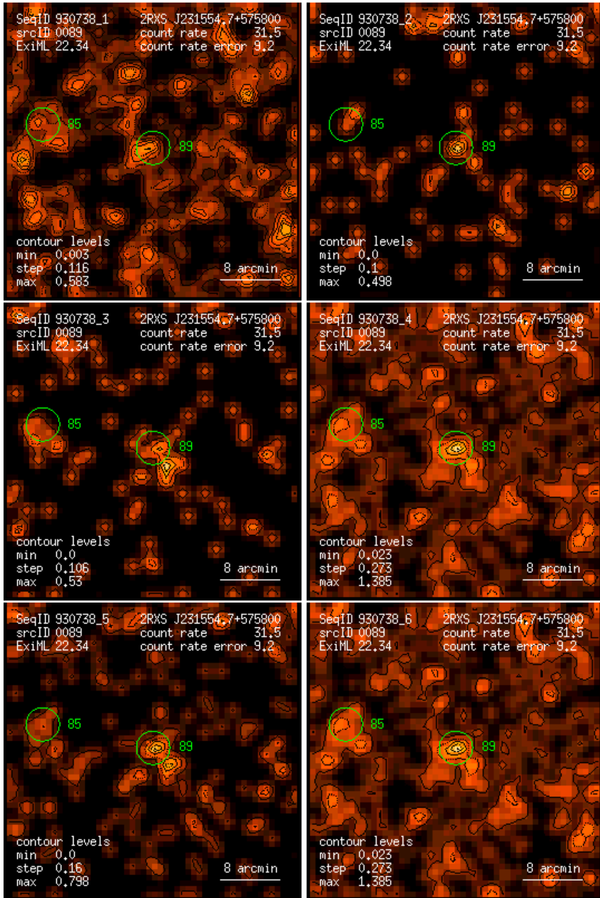
Figure 89: RASS 930738: detection 0089: band rate images, Gaussian filter: (1) PSPC channels 11 – 41, (2) 52 – 90, (3) 91 – 201, (4) 11 – 235, (5) 52 – 201, (6) 11 – 201. Broad band rates in counts/ks. Band rate contour levels in counts/ks/arcmin 2 .
