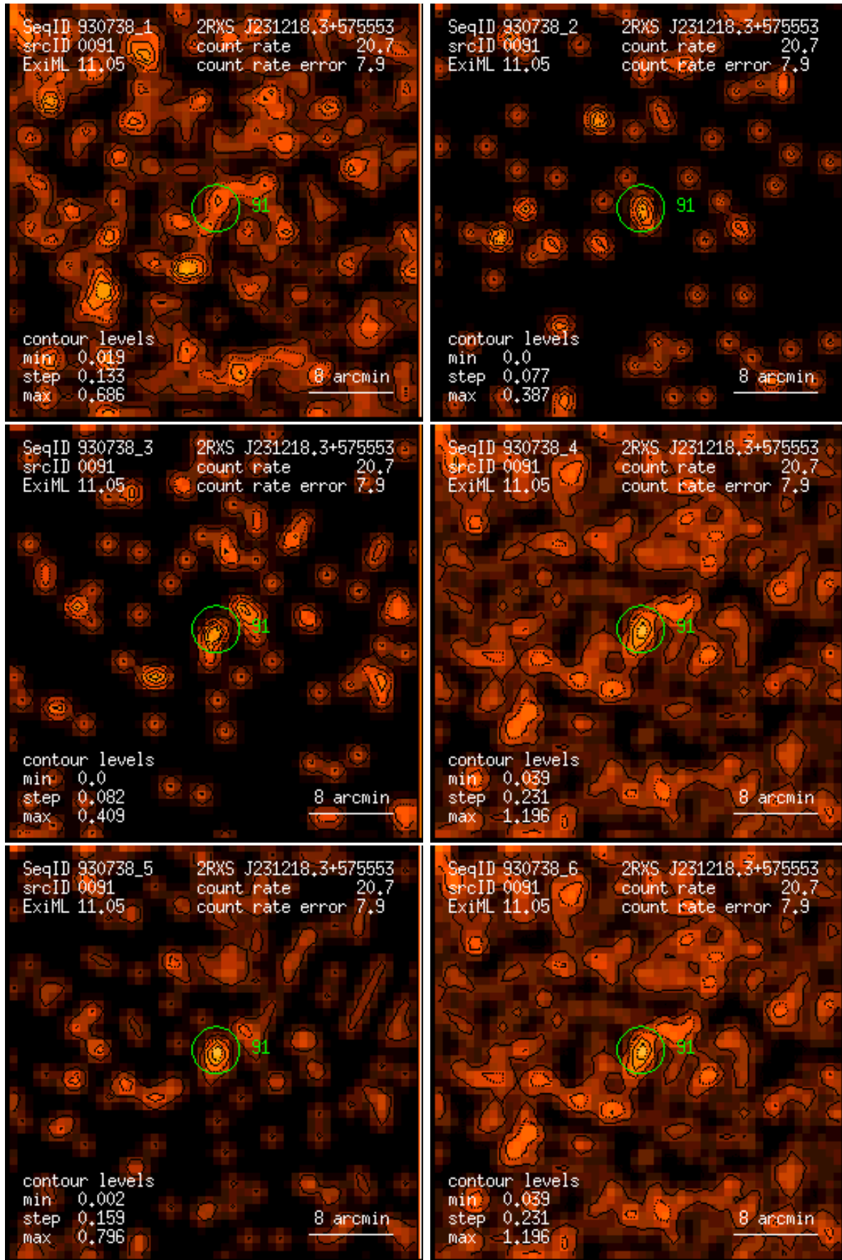
Figure 91: RASS 930738: detection 0091: band rate images, Gaussian filter: (1) PSPC channels 11 – 41, (2) 52 – 90, (3) 91 – 201, (4) 11 – 235, (5) 52 – 201, (6) 11 – 201. Broad band rates in counts/ks. Band rate contour levels in counts/ks/arcmin 2 .
