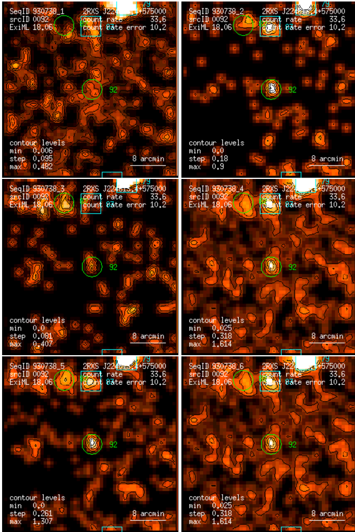
Figure 92: RASS 930738: detection 0092: band rate images, Gaussian filter: (1) PSPC channels 11 – 41, (2) 52 – 90, (3) 91 – 201, (4) 11 – 235, (5) 52 – 201, (6) 11 – 201. Broad band rates in counts/ks. Band rate contour levels in counts/ks/arcmin 2 .
