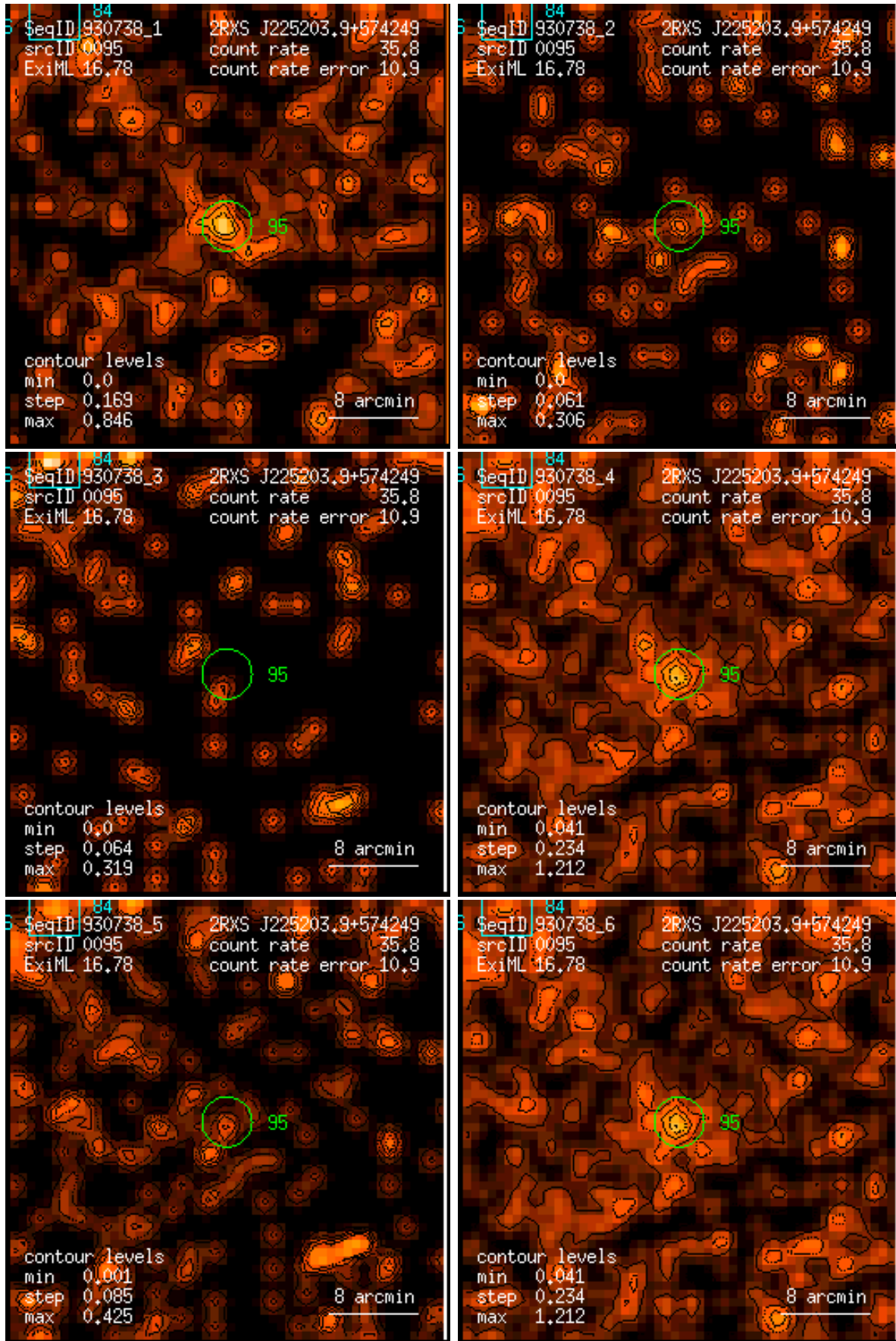
Figure 95: RASS 930738: detection 0095: band rate images, Gaussian filter: (1) PSPC channels 11 – 41, (2) 52 – 90, (3) 91 – 201, (4) 11 – 235, (5) 52 – 201, (6) 11 – 201. Broad band rates in counts/ks. Band rate contour levels in counts/ks/arcmin 2 .
