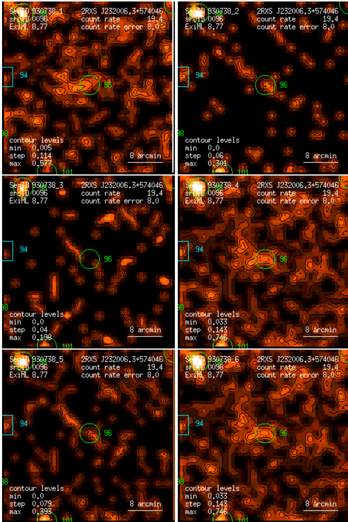
Figure 96: RASS 930738: detection 0096: band rate images, Gaussian filter: (1) PSPC channels 11 – 41, (2) 52 – 90, (3) 91 – 201, (4) 11 – 235, (5) 52 – 201, (6) 11 – 201. Broad band rates in counts/ks. Band rate contour levels in counts/ks/arcmin 2 .
