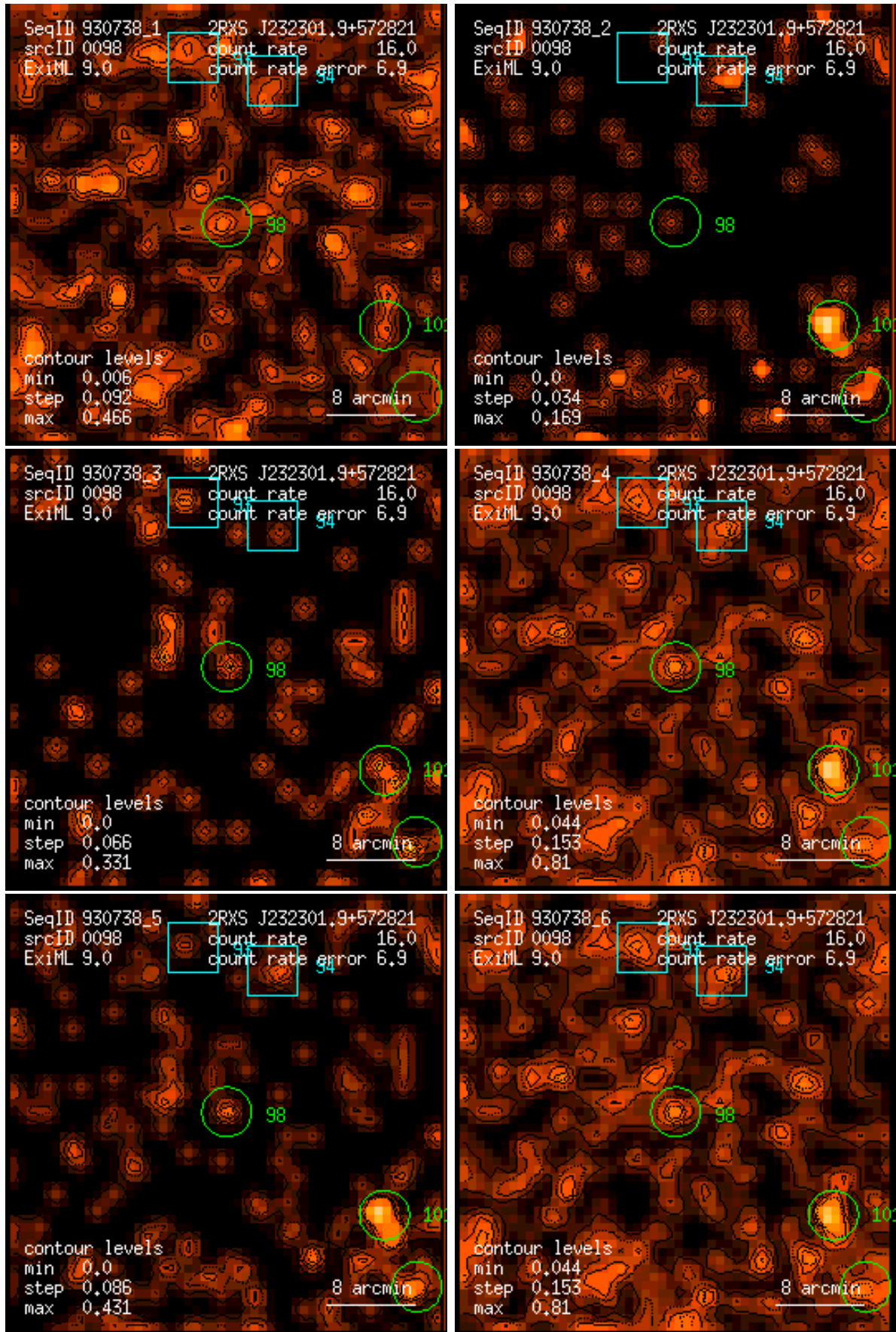
Figure 98: RASS 930738: detection 0098: band rate images, Gaussian filter: (1) PSPC channels 11 – 41, (2) 52 – 90, (3) 91 – 201, (4) 11 – 235, (5) 52 – 201, (6) 11 – 201. Broad band rates in counts/ks. Band rate contour levels in counts/ks/arcmin 2 .
