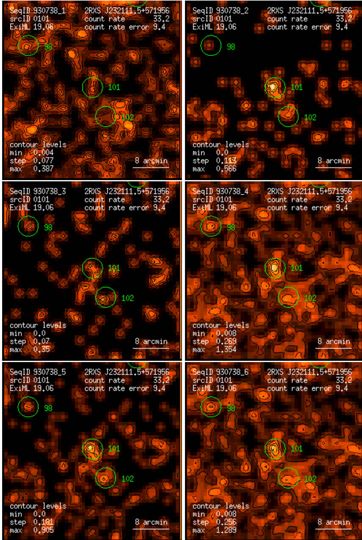
Figure 101: RASS 930738: detection 0101: band rate images, Gaussian filter: (1) PSPC channels 11 – 41, (2) 52 – 90, (3) 91 – 201, (4) 11 – 235, (5) 52 – 201, (6) 11 – 201. Broad band rates in counts/ks. Band rate contour levels in counts/ks/arcmin 2 .
