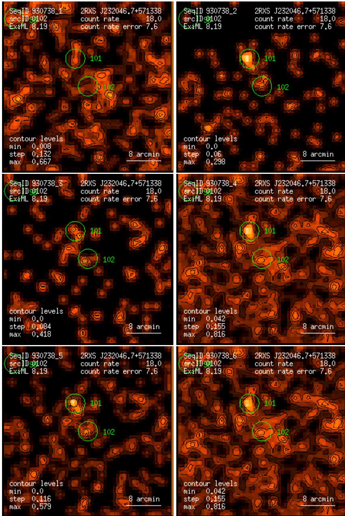
Figure 102: RASS 930738: detection 0102: band rate images, Gaussian filter: (1) PSPC channels 11 – 41, (2) 52 – 90, (3) 91 – 201, (4) 11 – 235, (5) 52 – 201, (6) 11 – 201. Broad band rates in counts/ks. Band rate contour levels in counts/ks/arcmin 2 .
