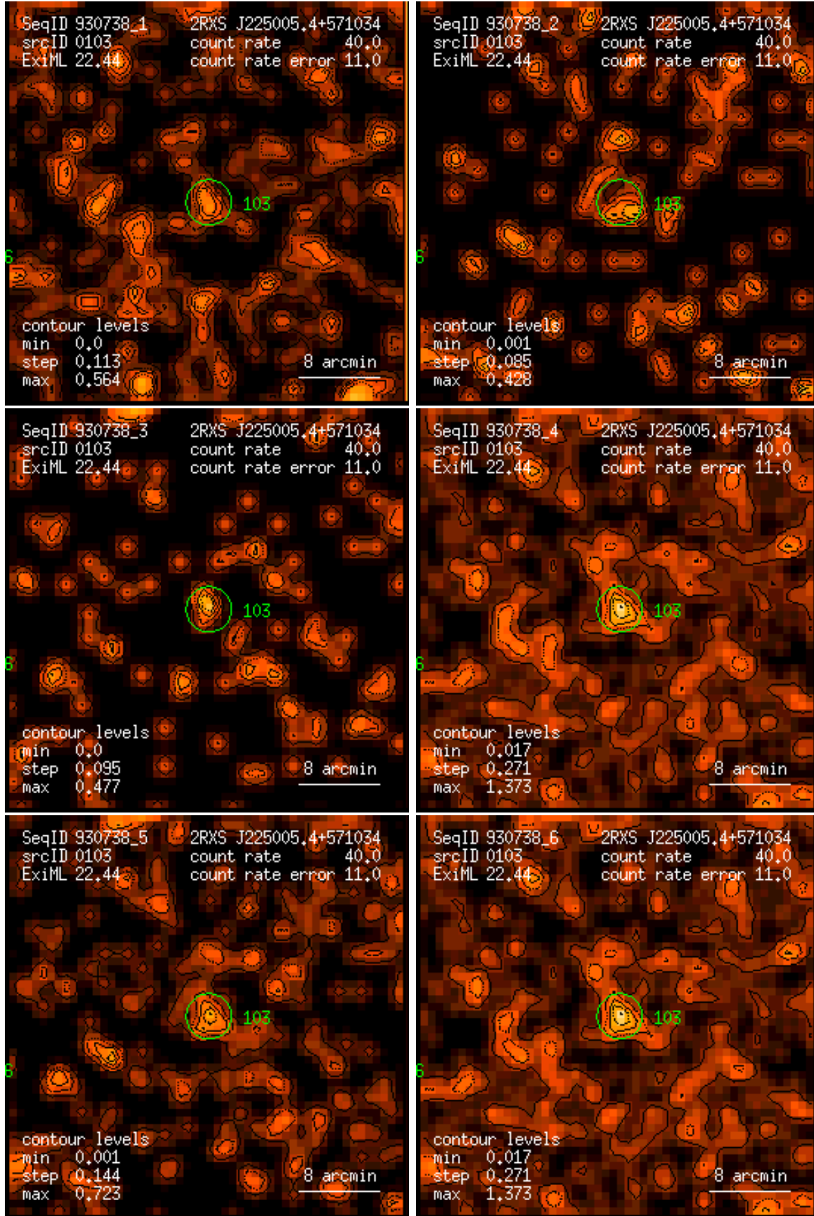
Figure 103: RASS 930738: detection 0103: band rate images, Gaussian filter: (1) PSPC channels 11 – 41, (2) 52 – 90, (3) 91 – 201, (4) 11 – 235, (5) 52 – 201, (6) 11 – 201. Broad band rates in counts/ks. Band rate contour levels in counts/ks/arcmin 2 .
