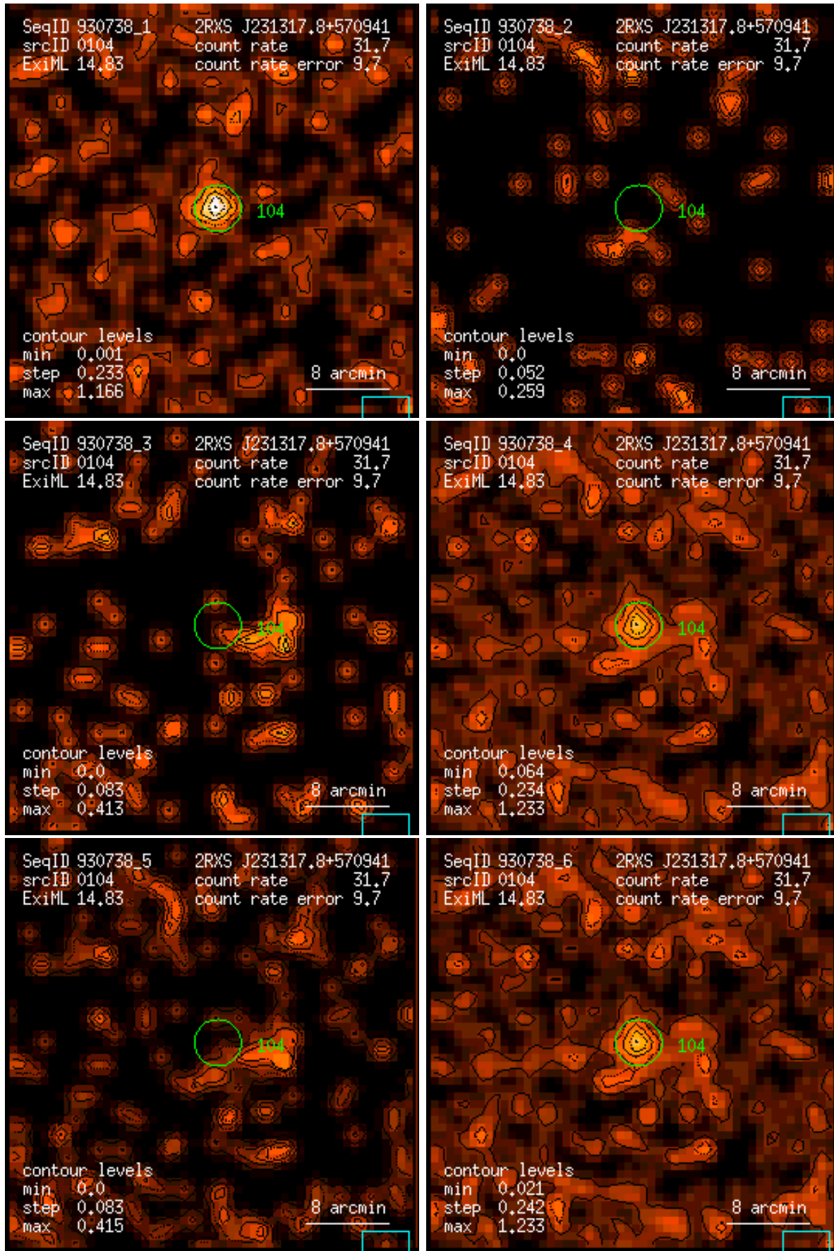
Figure 104: RASS 930738: detection 0104: band rate images, Gaussian filter: (1) PSPC channels 11 – 41, (2) 52 – 90, (3) 91 – 201, (4) 11 – 235, (5) 52 – 201, (6) 11 – 201. Broad band rates in counts/ks. Band rate contour levels in counts/ks/arcmin 2 .
