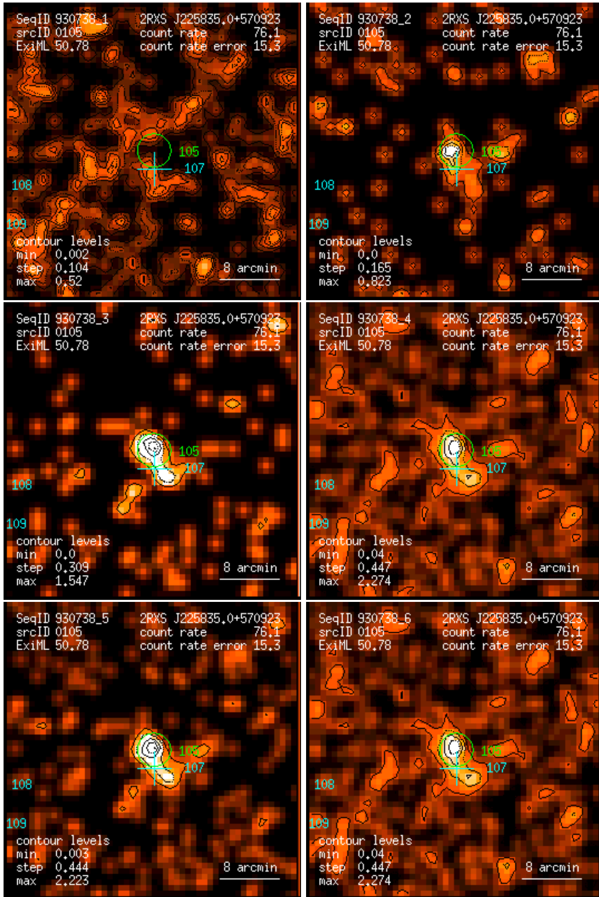
Figure 105: RASS 930738: detection 0105: band rate images, Gaussian filter: (1) PSPC channels 11 – 41, (2) 52 – 90, (3) 91 – 201, (4) 11 – 235, (5) 52 – 201, (6) 11 – 201. Broad band rates in counts/ks. Band rate contour levels in counts/ks/arcmin 2 .
