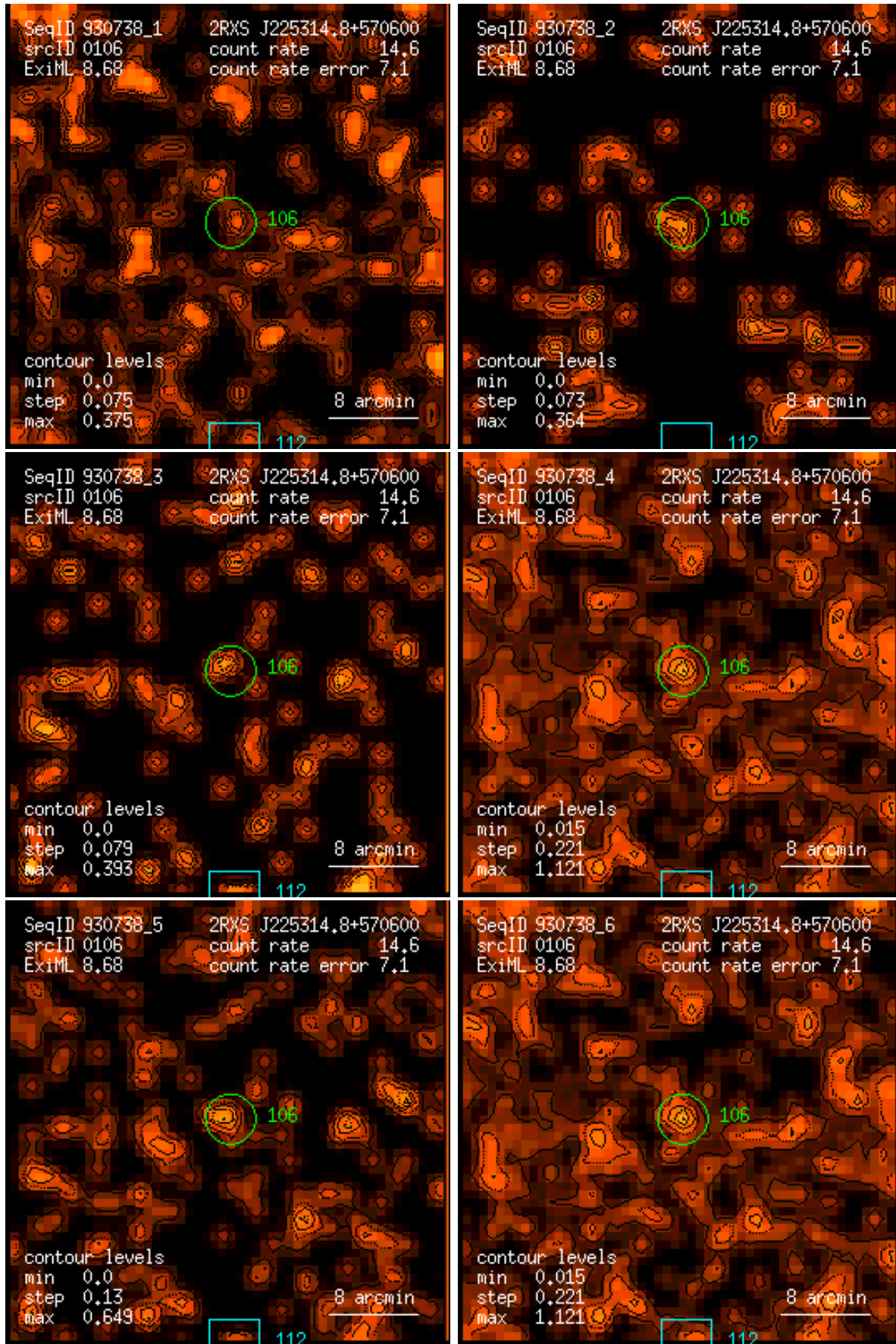
Figure 106: RASS 930738: detection 0106: band rate images, Gaussian filter: (1) PSPC channels 11 – 41, (2) 52 – 90, (3) 91 – 201, (4) 11 – 235, (5) 52 – 201, (6) 11 – 201. Broad band rates in counts/ks. Band rate contour levels in counts/ks/arcmin 2 .
